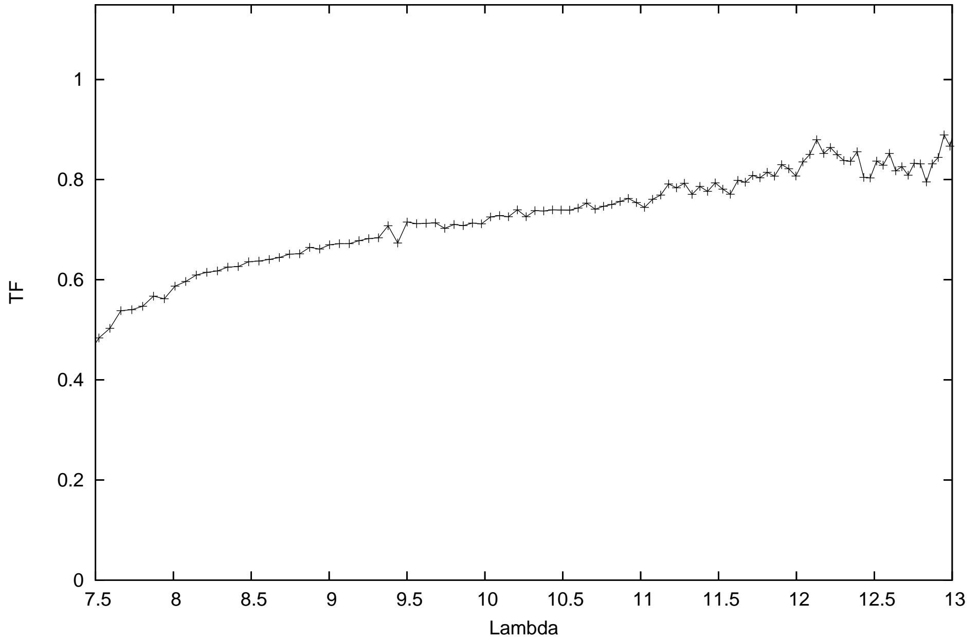
calHD167618_flux-1.82_diam11.66_r.MIDI.2013-10-06T00_41_28.000_C1B2
