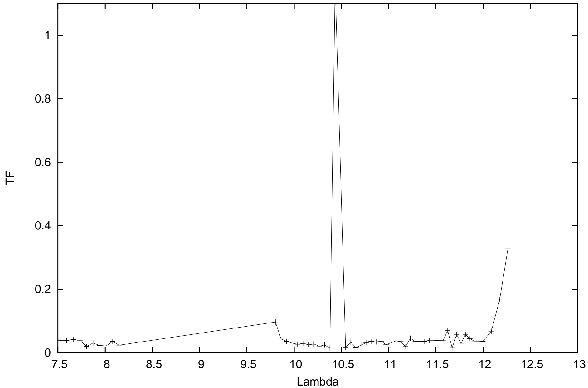
calHD167618_flux-1.82_diam11.66_r.MIDI.2013-10-01T23_37_05.000_H0C1
