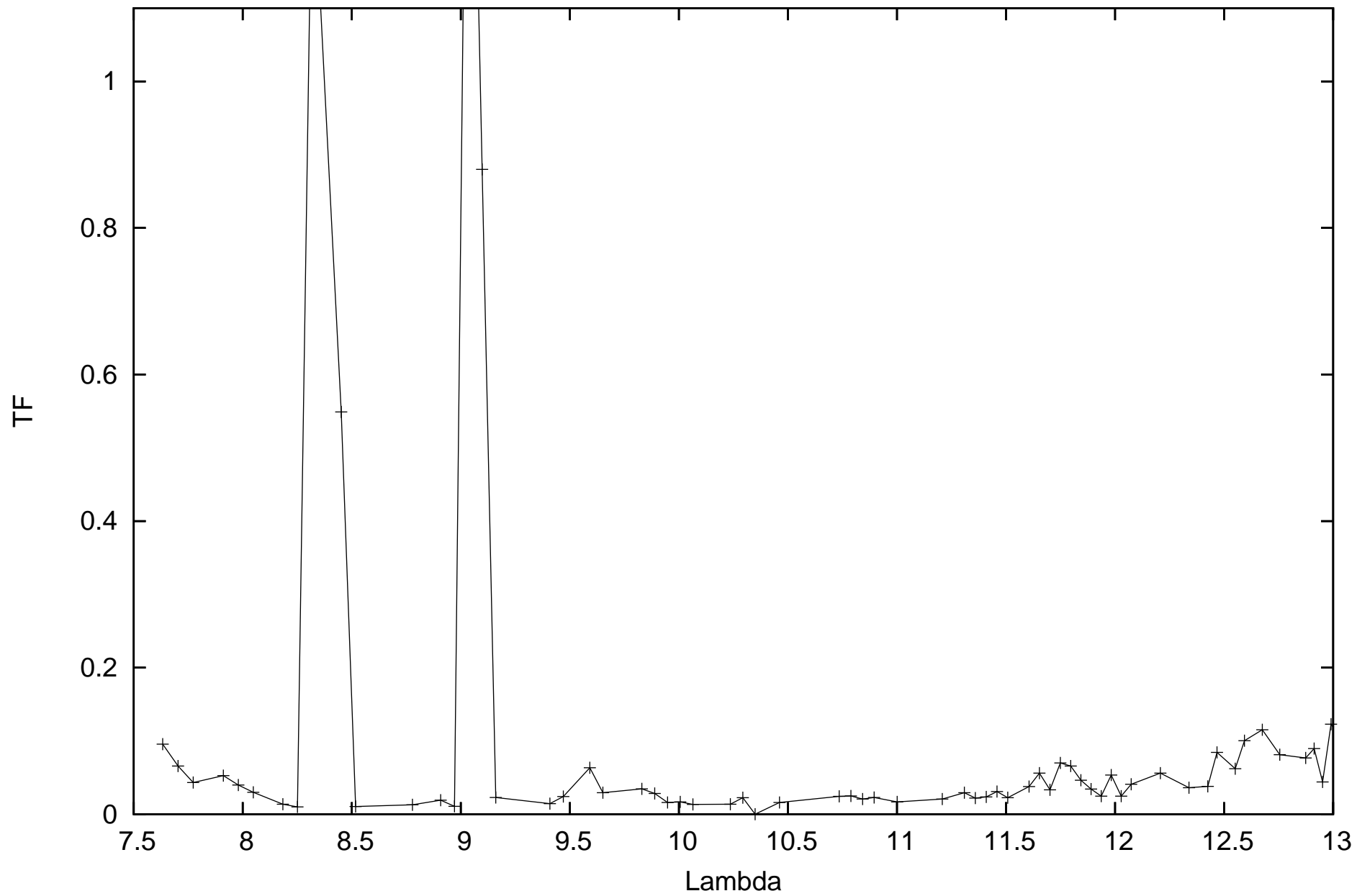
calHD167618_flux-1.82_diam11.66_r.MIDI.2013-07-30T07_40_03.113_D0B2
