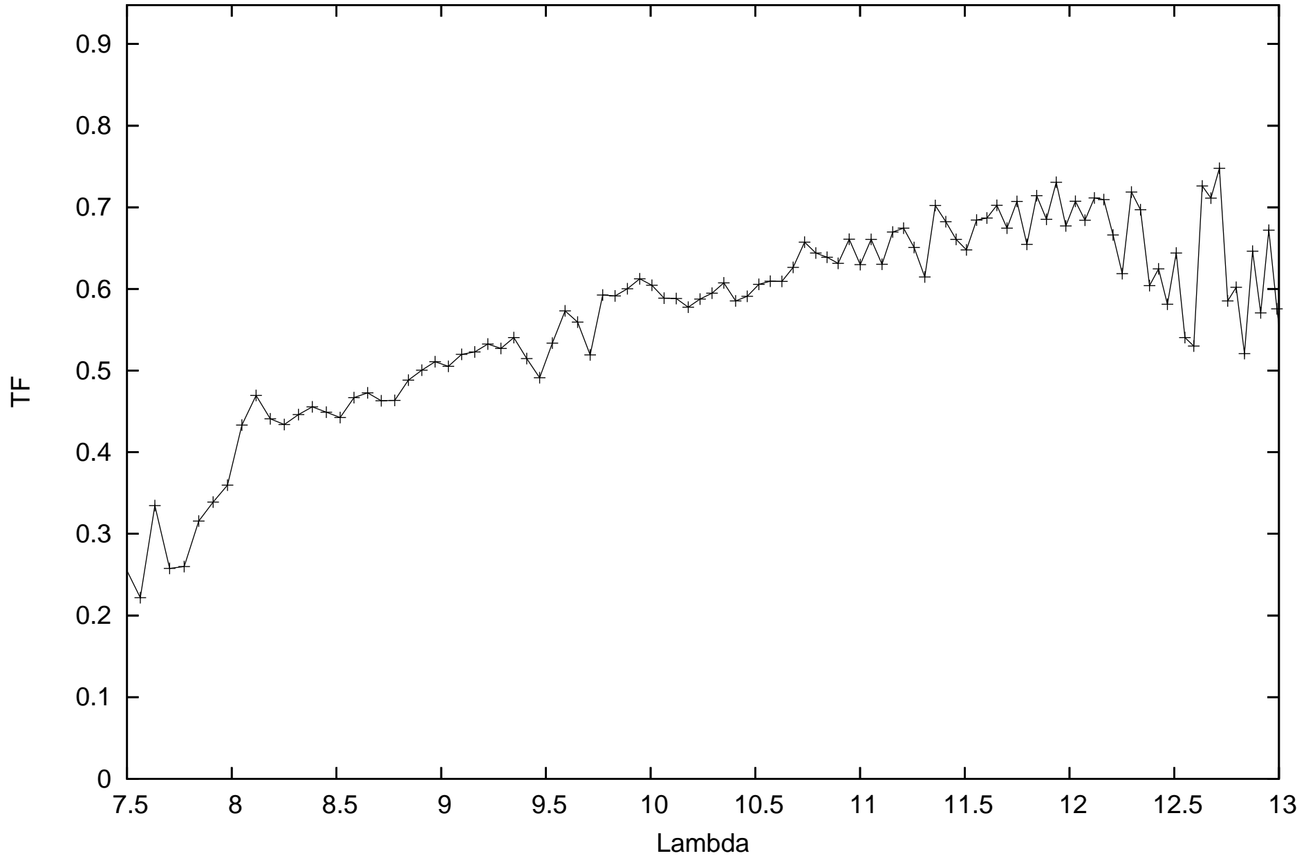
calHD167618_flux-1.82_diam11.66_r.MIDI.2013-07-30T06_58_08.112_B2A1
