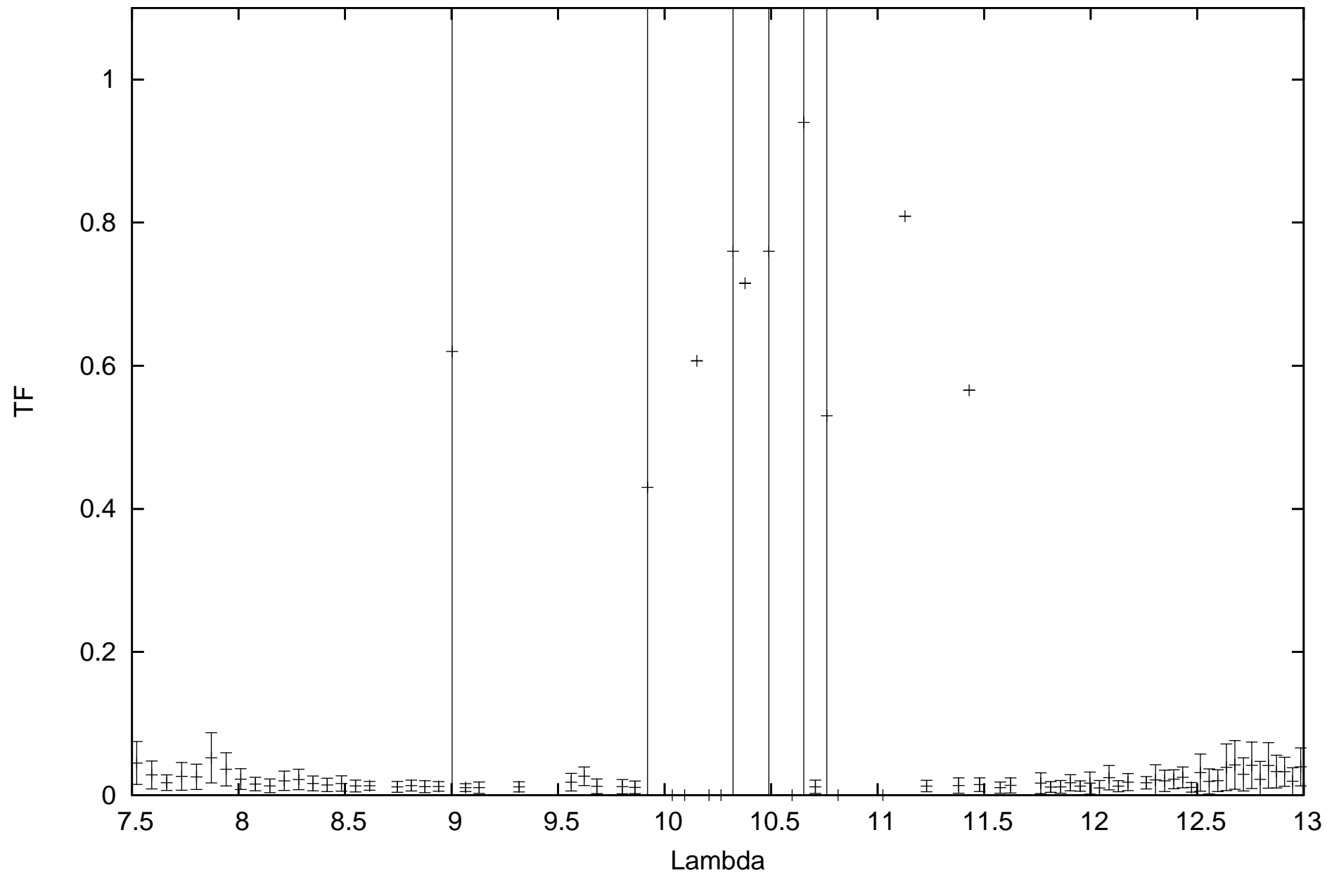
calHD167618_flux-1.82_diam11.66_r.MIDI.2013-07-01T06_13_33.000_D0A1
