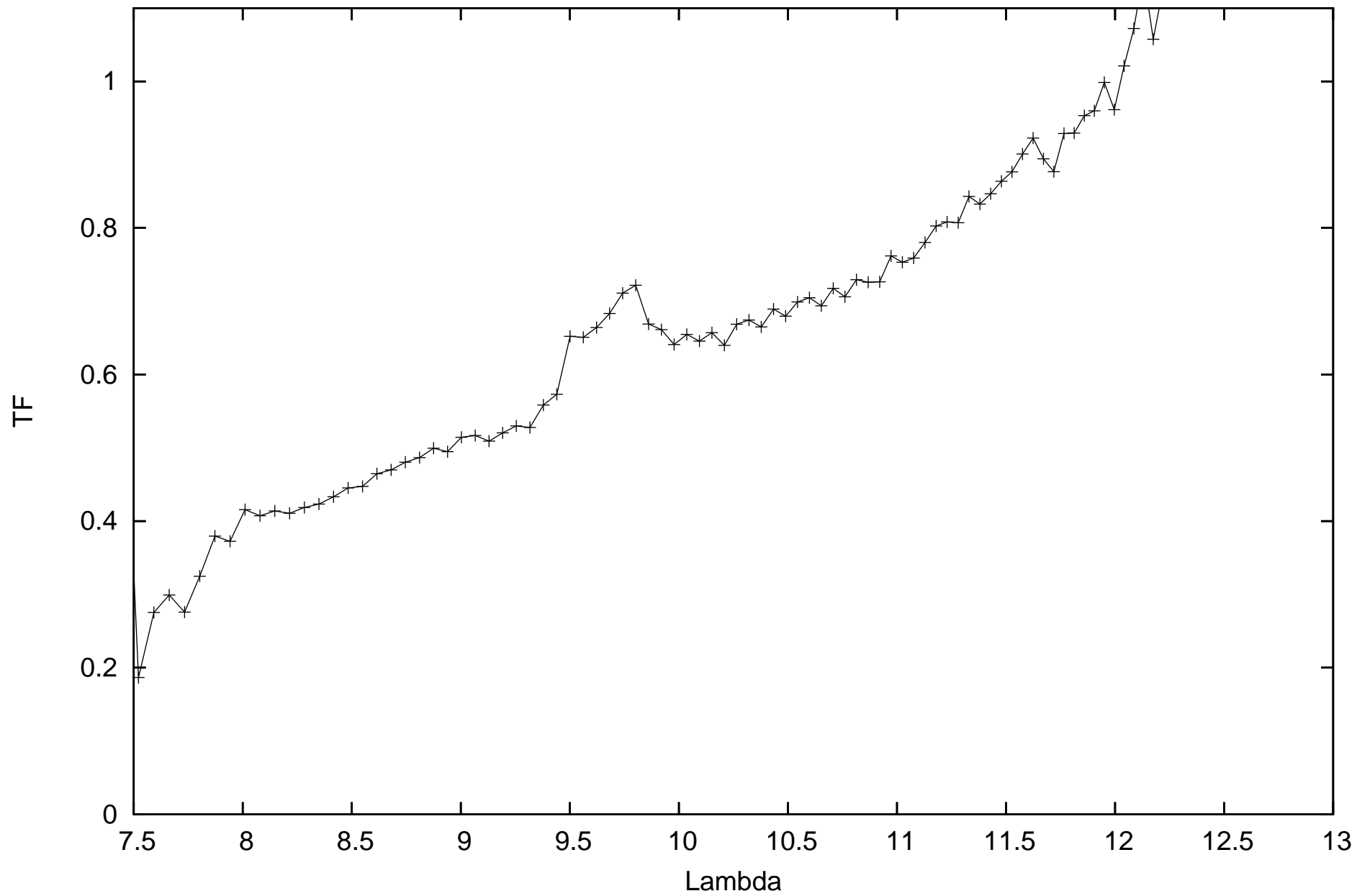
calHD167618_flux-1.82_diam11.66_r.MIDI.2013-06-12T08_48_50.000_D0H0
