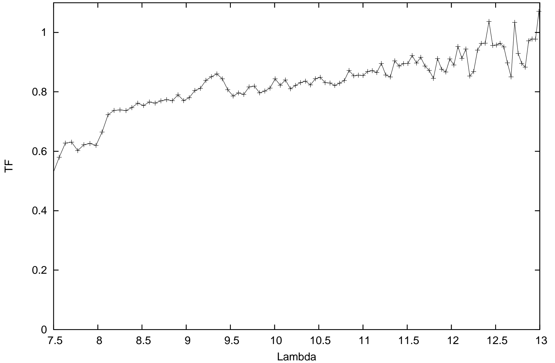
calHD167618_flux-1.82_diam11.66_r.MIDI.2013-04-16T08_38_37.113_D0A1
