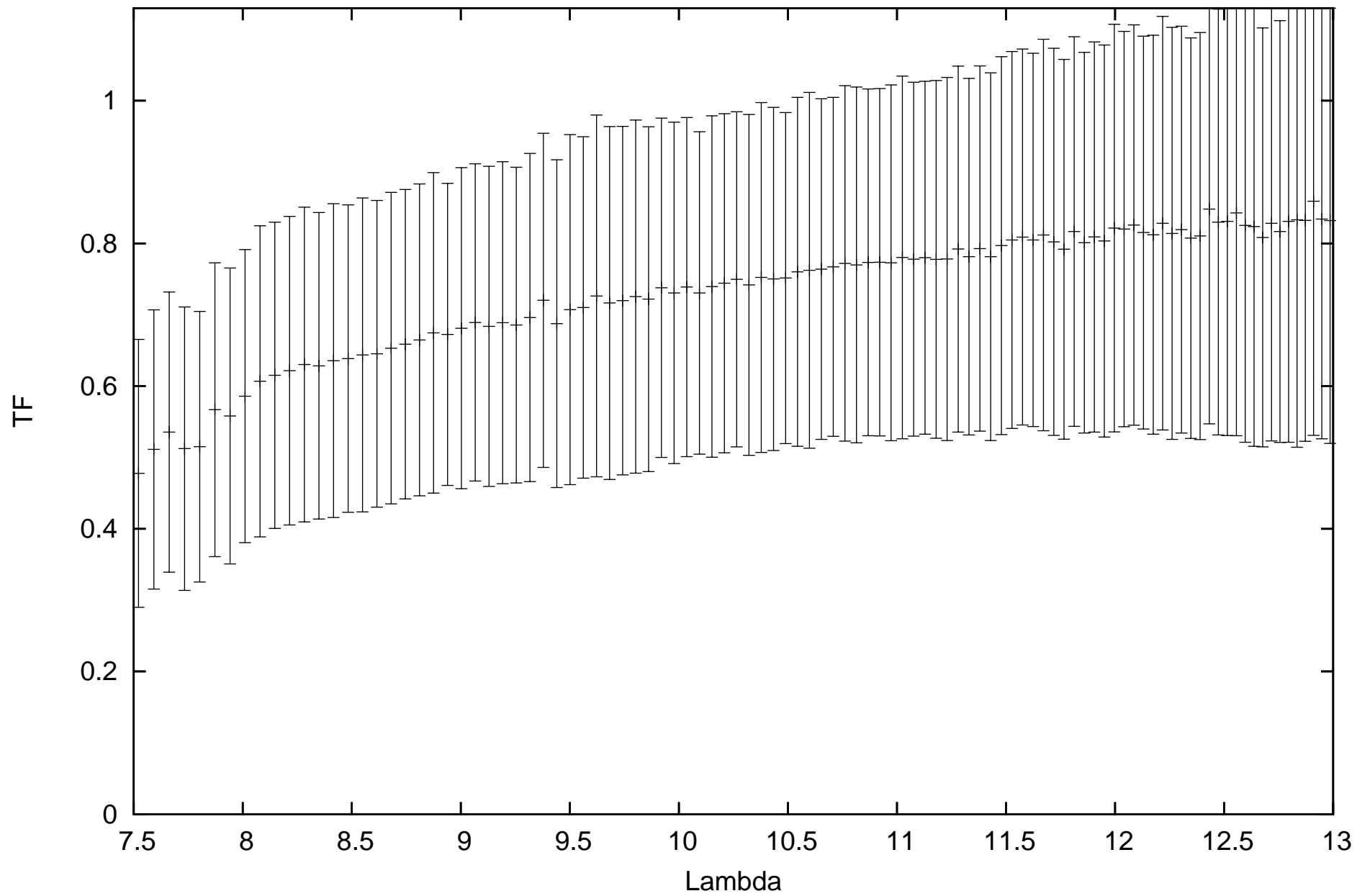
calHD137066_flux1.39_diam2.69_r.MIDI.2013-05-03T06_26_51.000_U1U2
