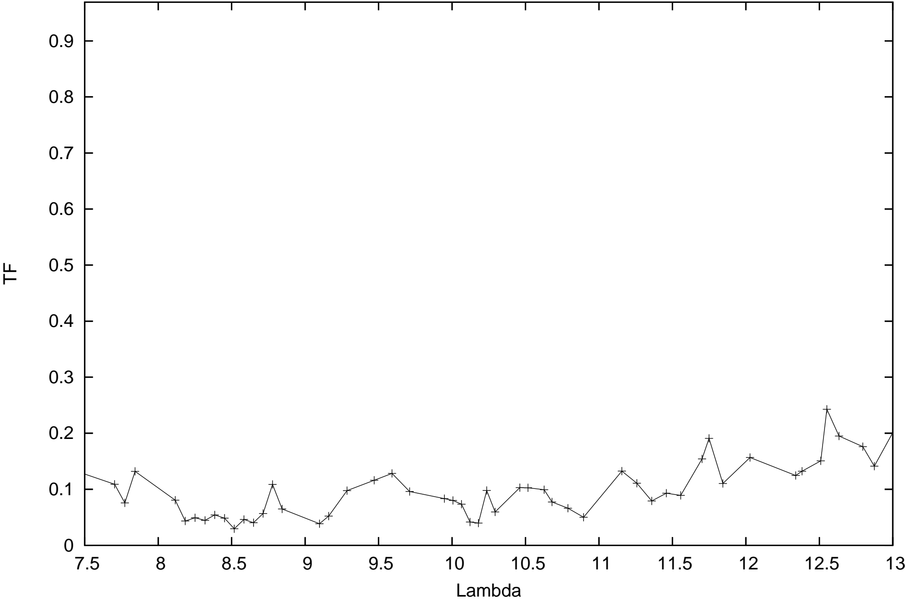
calHD107446_flux0.22_diam4.43_r.MIDI.2013-04-09T09_25_27.932_G111
