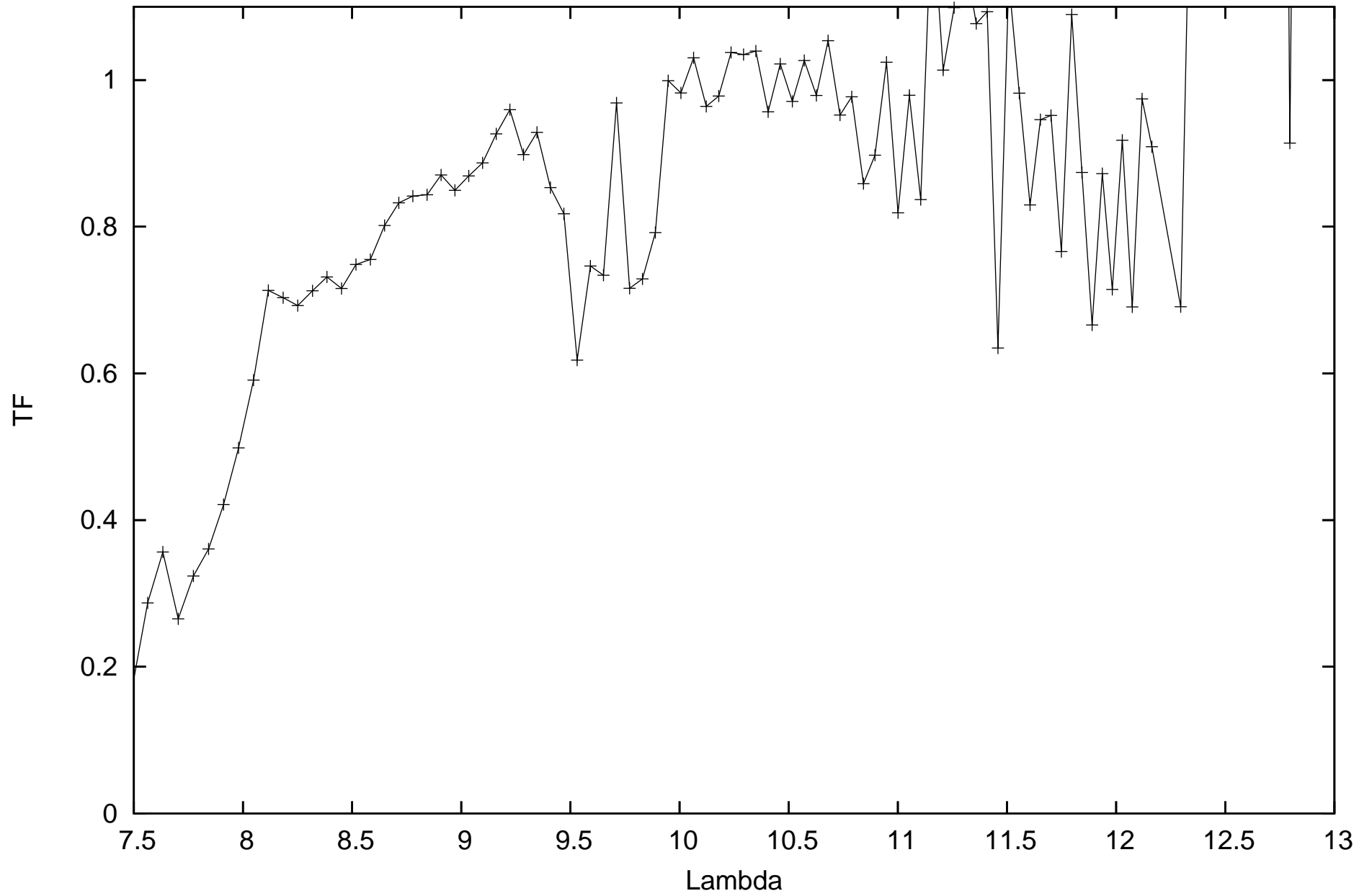
calHD107446_flux0.22_diam4.43_r.MIDI.2013-04-08T07_01_17.135_H0G1
