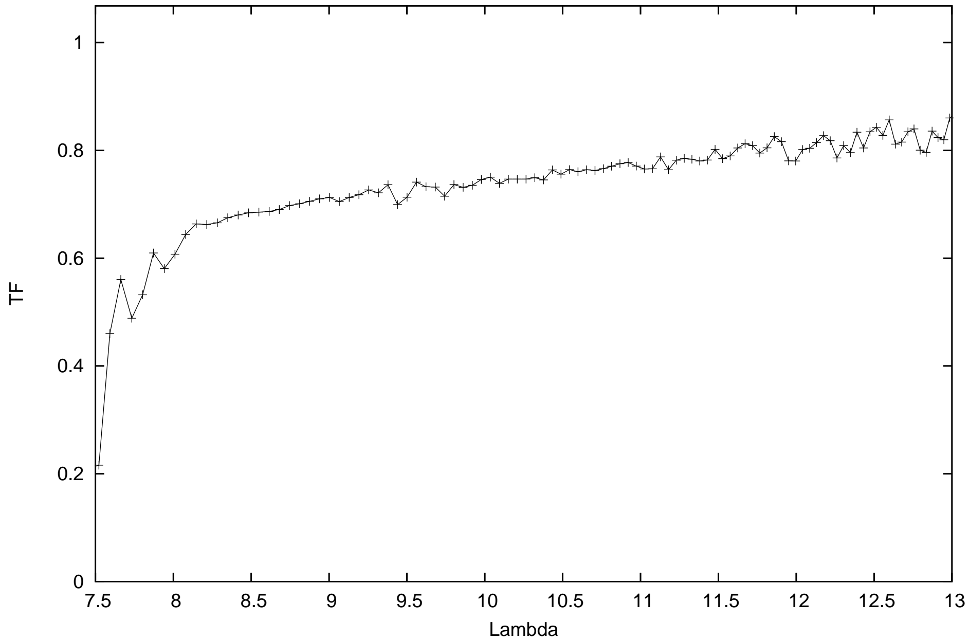
calHD102839_flux1.69_diam2.03_r.MIDI.2013-03-03T09_05_00.000_U2U4
