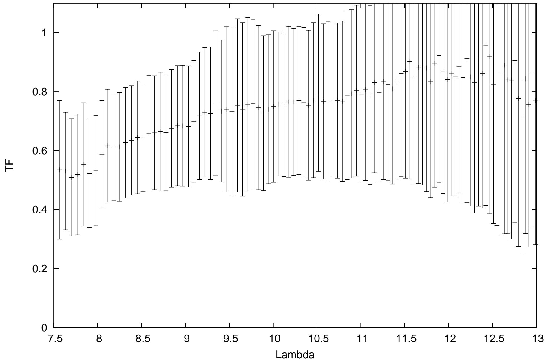
calHD81797_flux-1.49_diam9.14_r.MIDI.2013-12-31T07_39_37.932_G1A1
