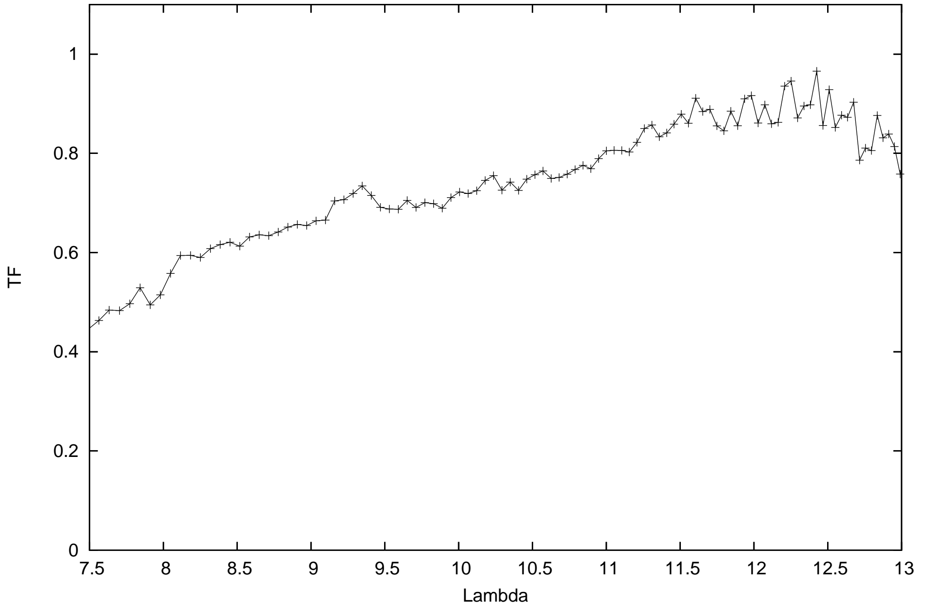
calHD81797_flux-1.49_diam9.14_r.MIDI.2013-12-31T06_56_09.135_K0G1
