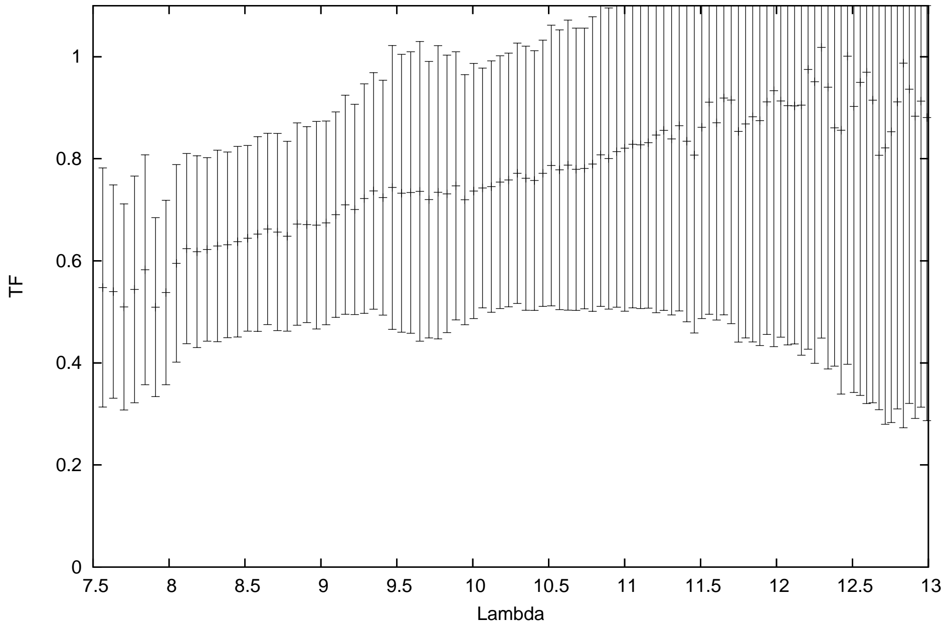
calHD81797_flux-1.49_diam9.14_r.MIDI.2013-12-31T06_36_30.932_G1A1
