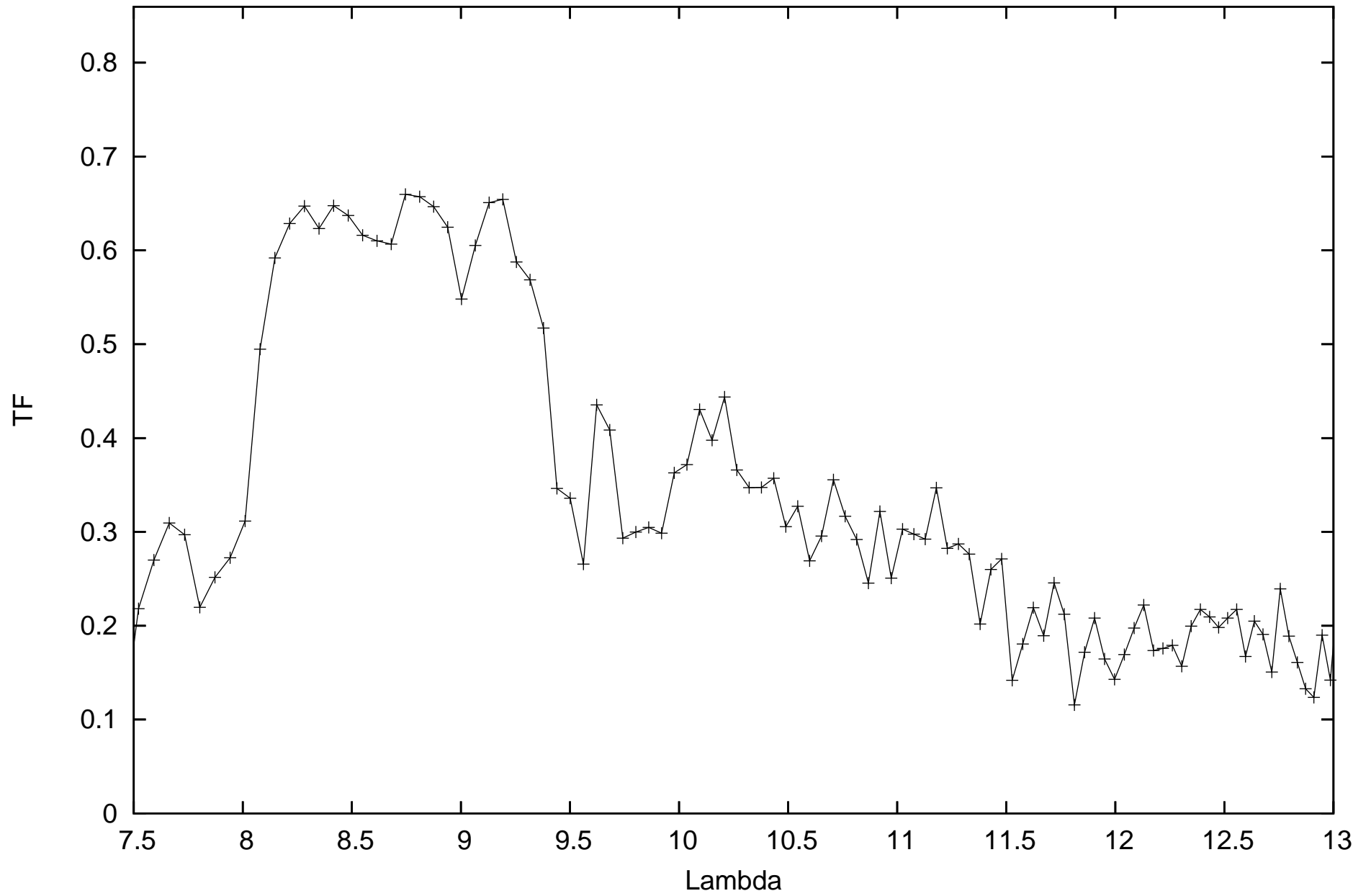
calHD98292_flux0.92_diam3.35_r.MIDI.2013-12-30T08_46_54.000_K0J3
