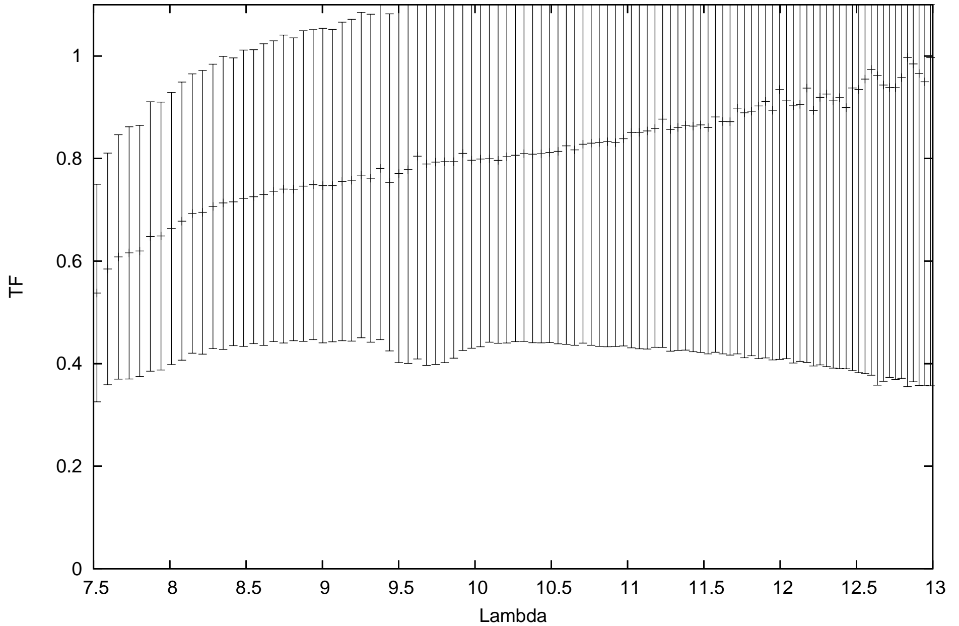
calHIP24197_flux1.37991_diam2.442016_r.MIDI.2013-12-20T01_53_54.000_U3U4
