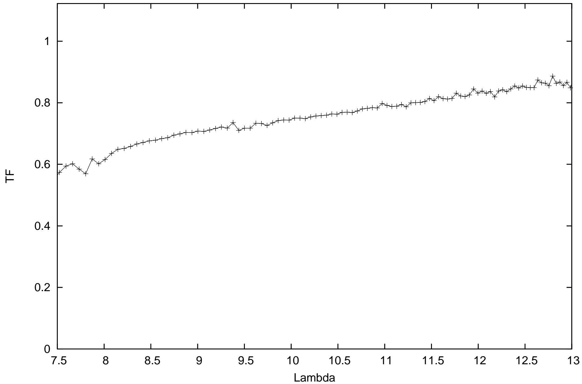
calHIP7588_flux0.936365_diam1.68_r.MIDI.2013-12-16T00_21_19.000_U2U3
