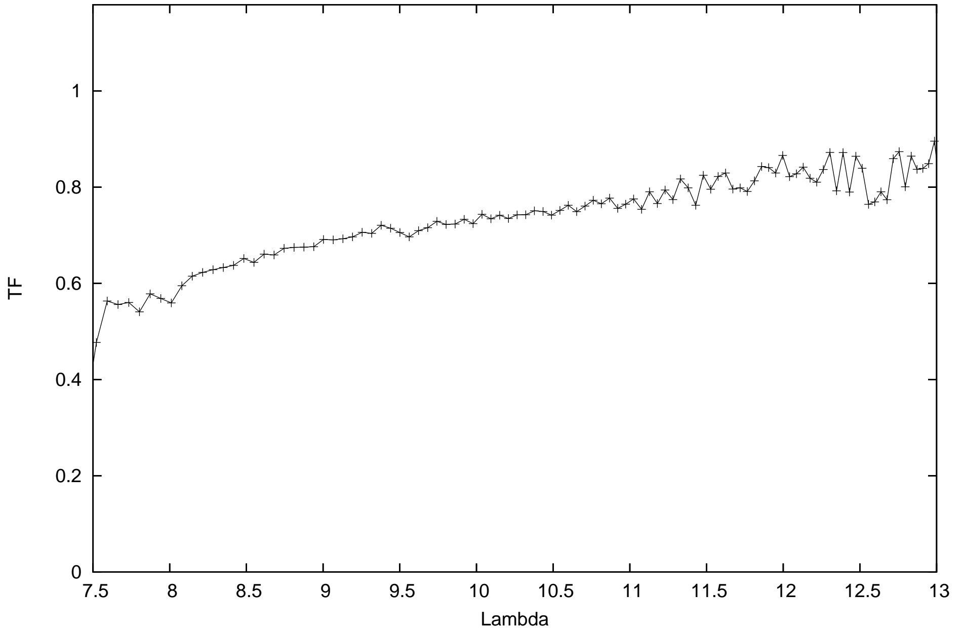
calHIP27938_flux1.62718_diam2.214782_r.MIDI.2013-12-16T03_26_01.000_U2U3
