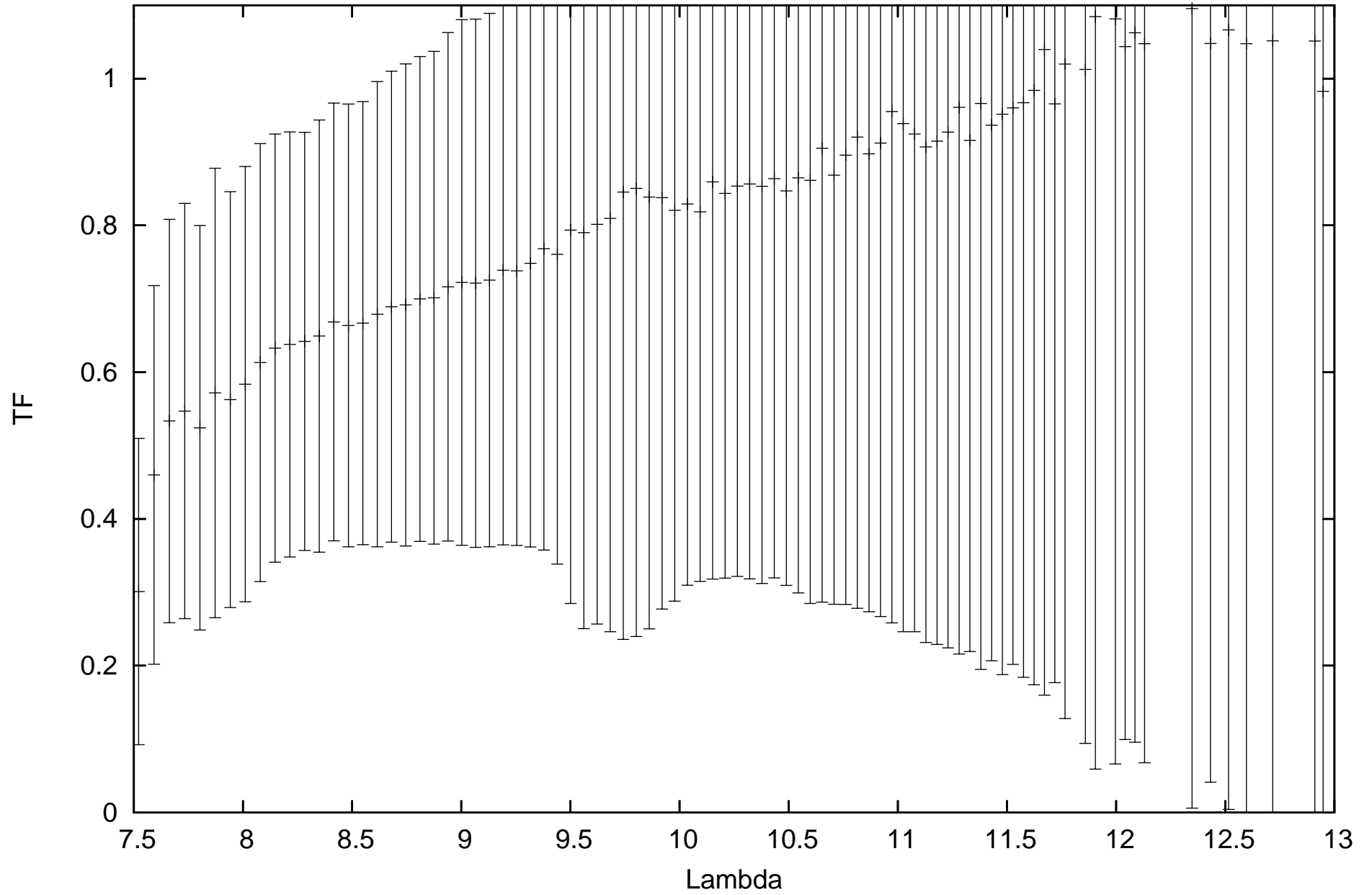
calHIP27938_flux1.62718_diam2.214782_r.MIDI.2013-12-16T02_30_40.000_U2U3
