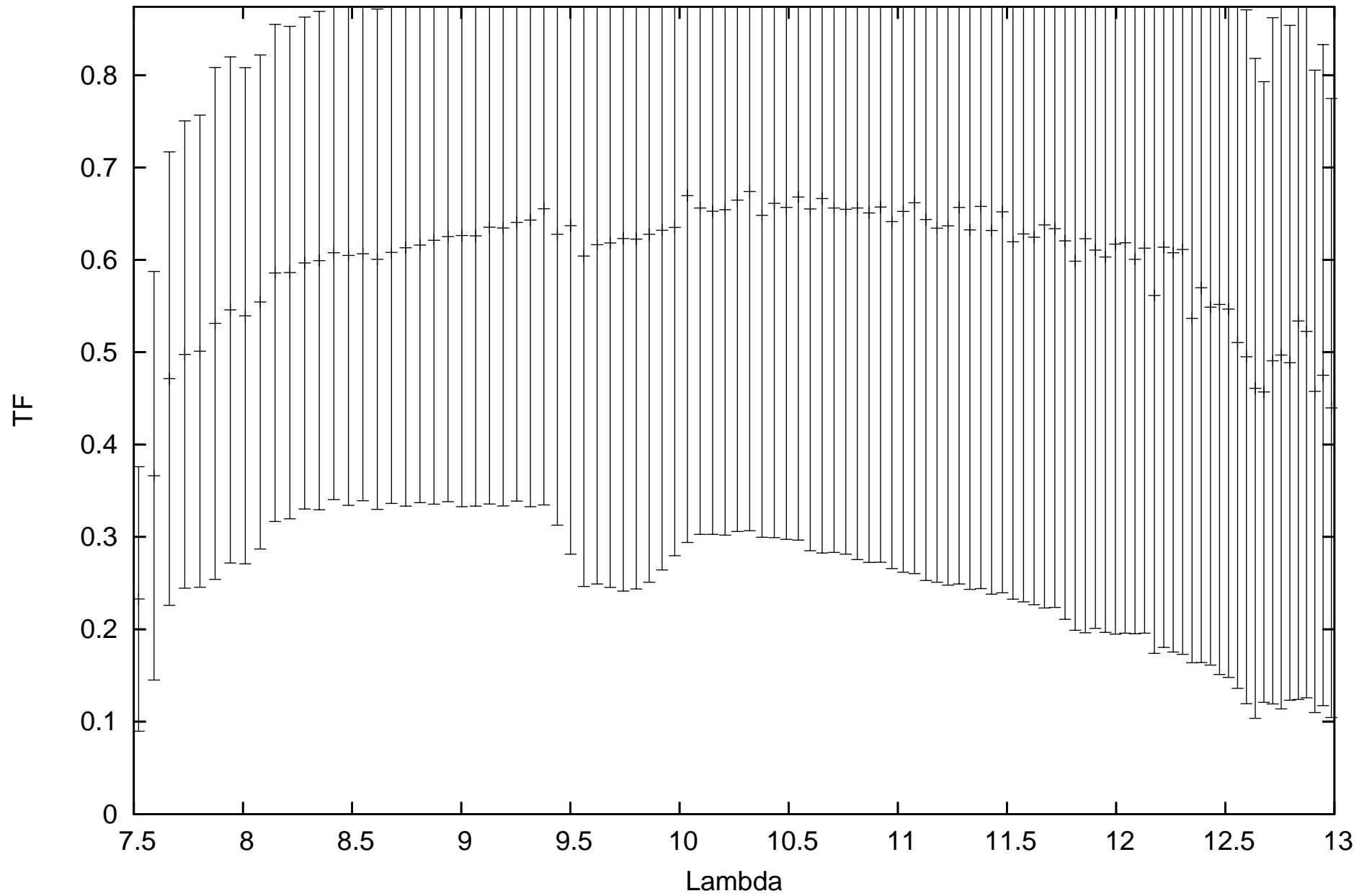
calHIP25583_flux1.57349_diam2.419193_r.MIDI.2013-12-16T04_22_44.000_U1U3
