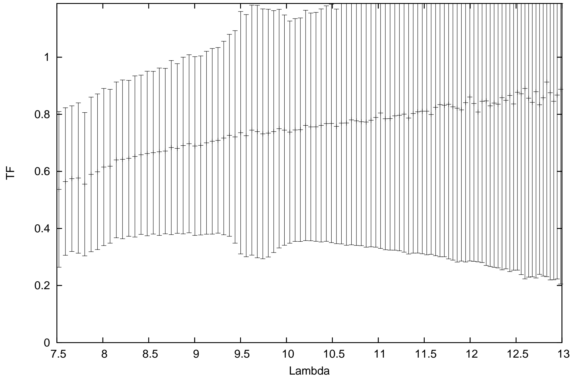
calHIP110997_flux1.58908_diam2.11_r.MIDI.2013-12-15T00_34_13.000_U1U2
