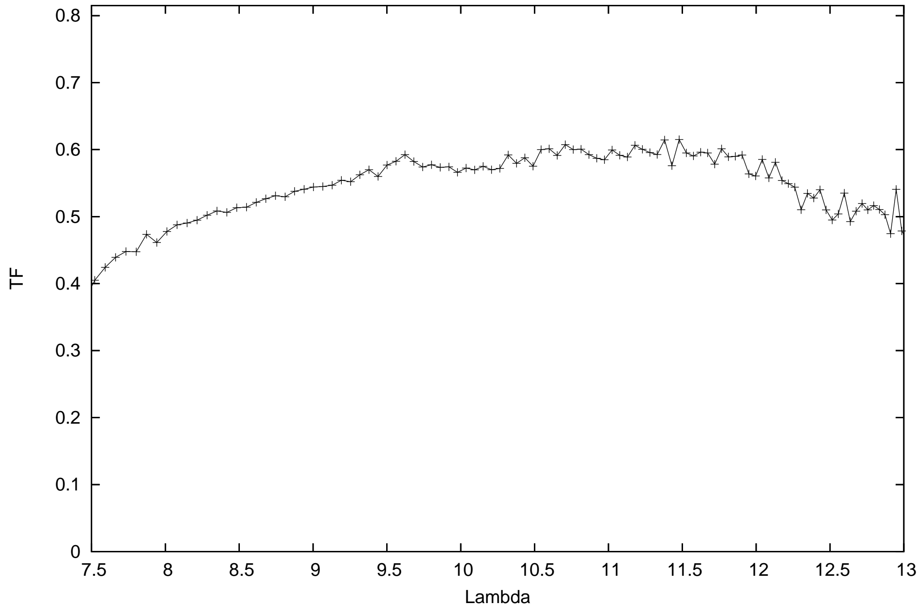
calHD48915_flux-1.39_diam6.09_r.MIDI.2013-12-03T07_15_09.000_B2A1
