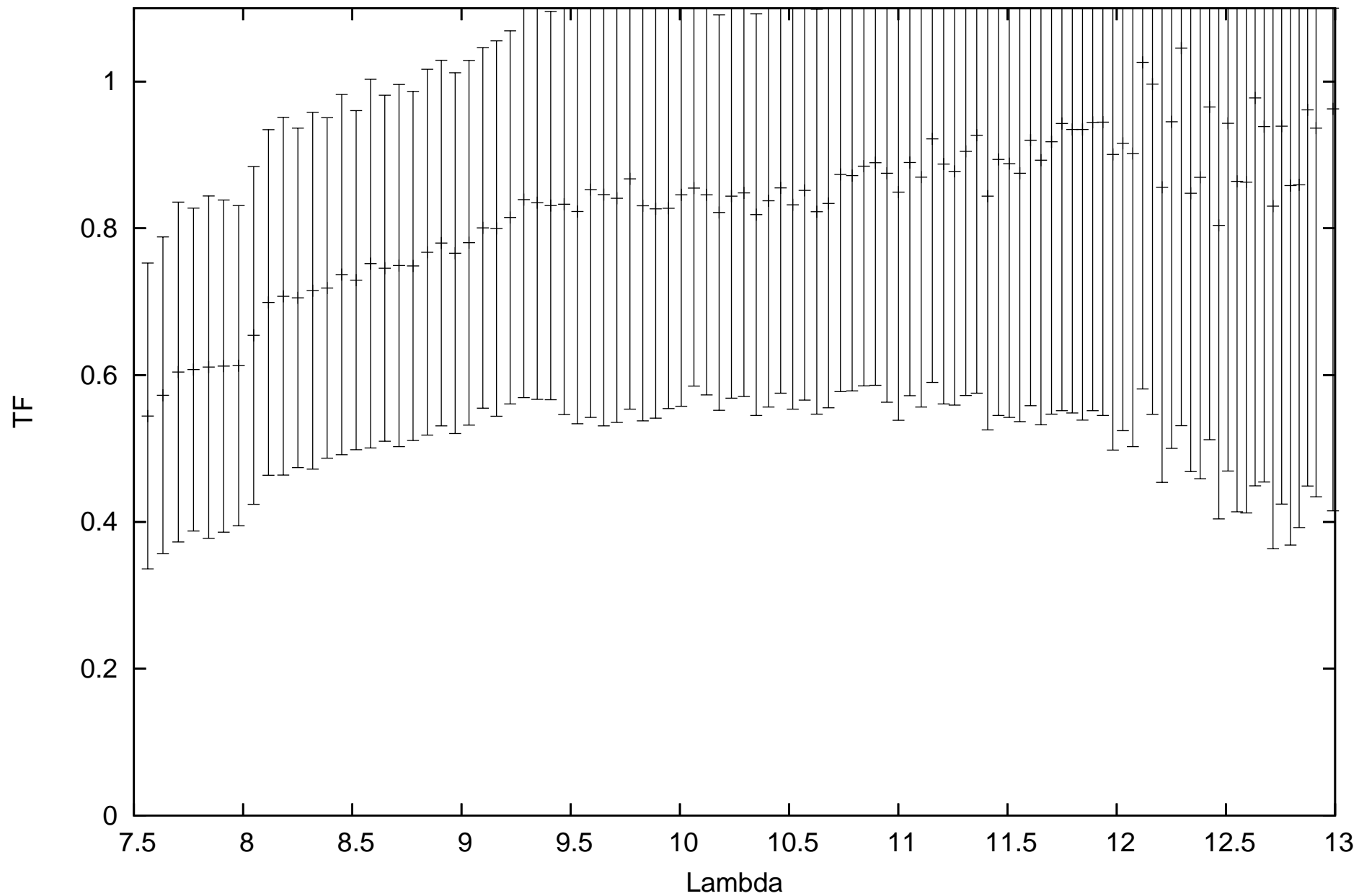
calHD48915_flux-1.39_diam6.09_r.MIDI.2013-11-17T08_40_35.932_B2A1
