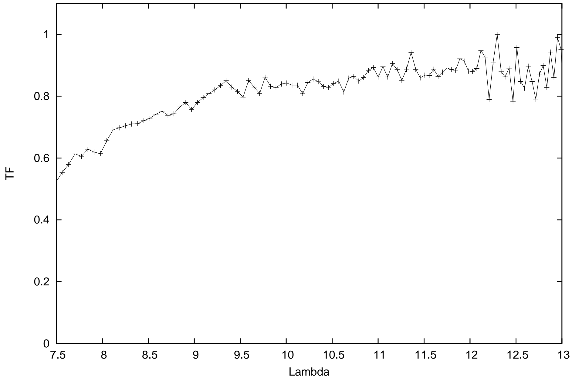
calHD48915_flux-1.39_diam6.09_r.MIDI.2013-11-17T08_11_03.932_B2A1
