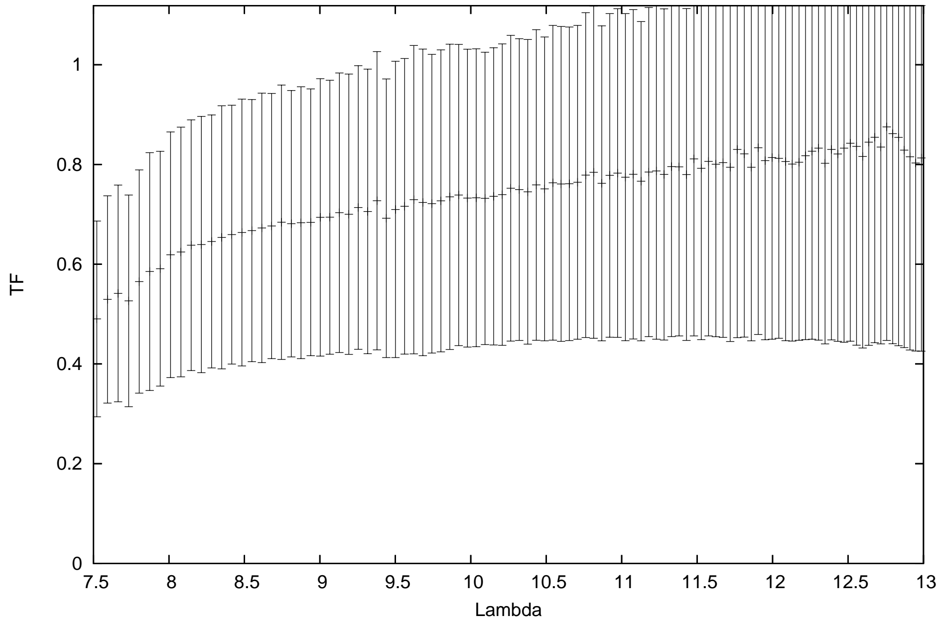
calHIP110997_flux1.58908_diam2.11_r.MIDI.2013-10-20T03_06_21.000_U1U3
