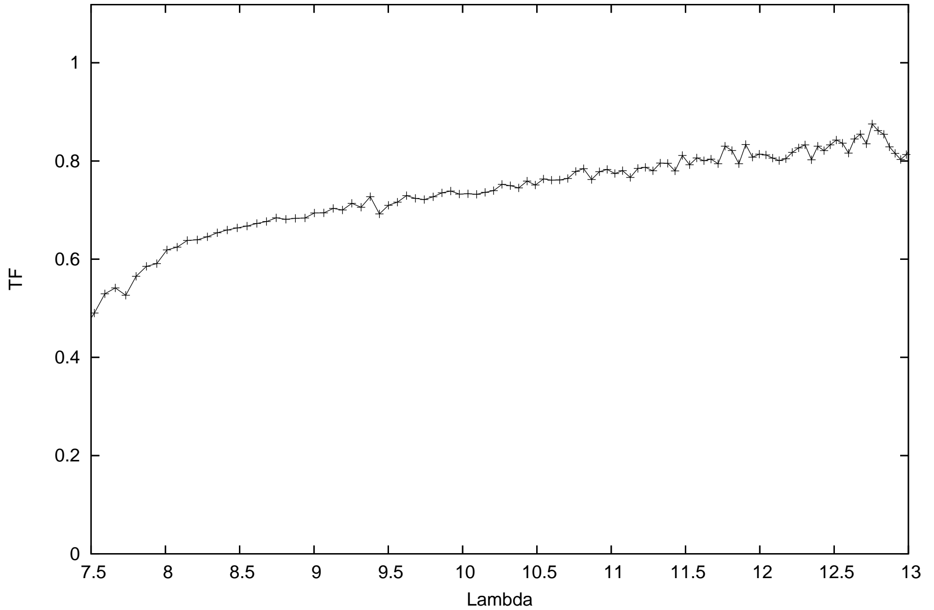
calHIP110997_flux1.58908_diam2.11_r.MIDI.2013-10-20T03_06_21.000_U1U3
