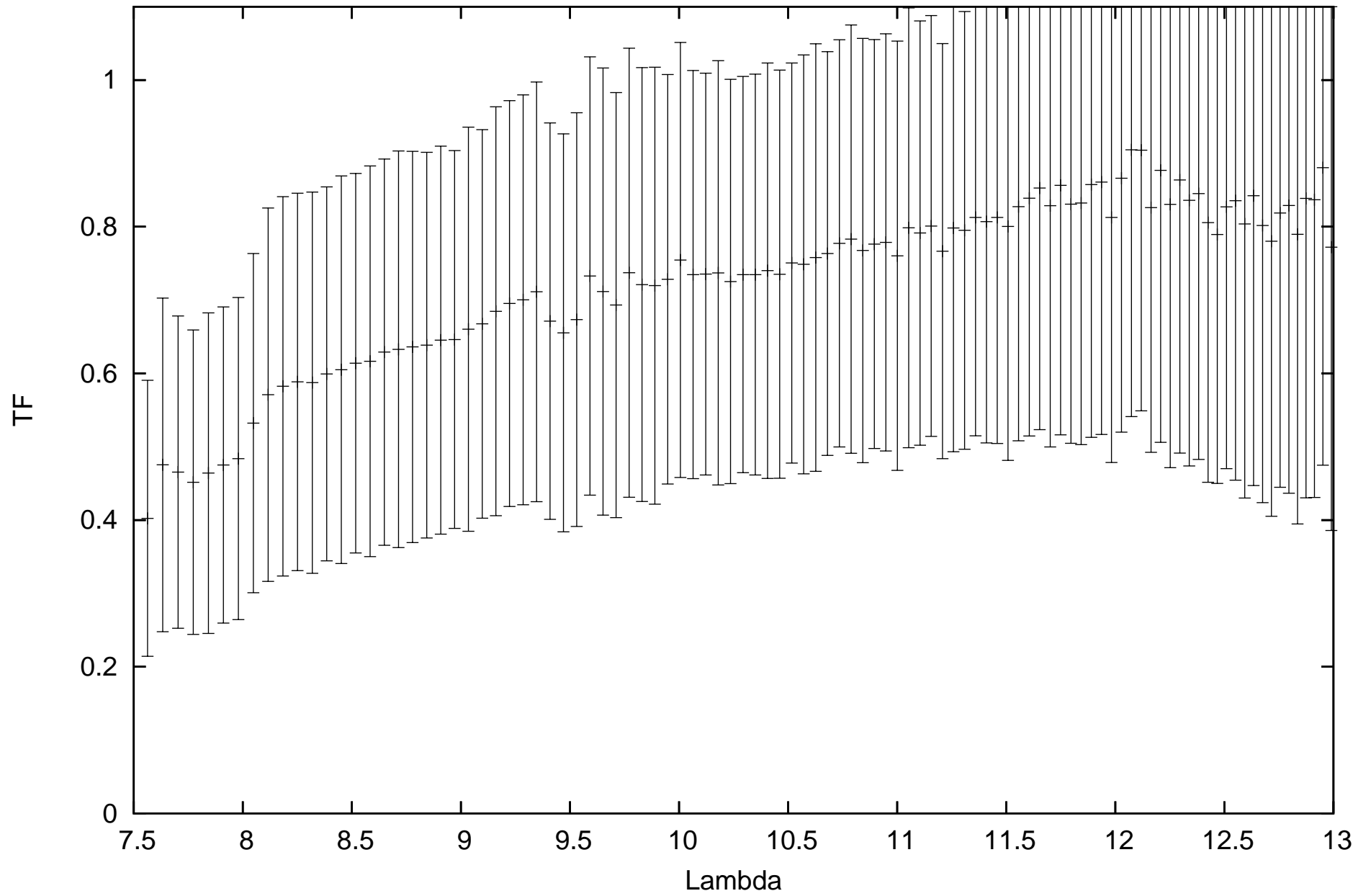
calHD167618_flux-1.82_diam11.66_r.MIDI.2013-10-06T00_50_10.113_C1B2
