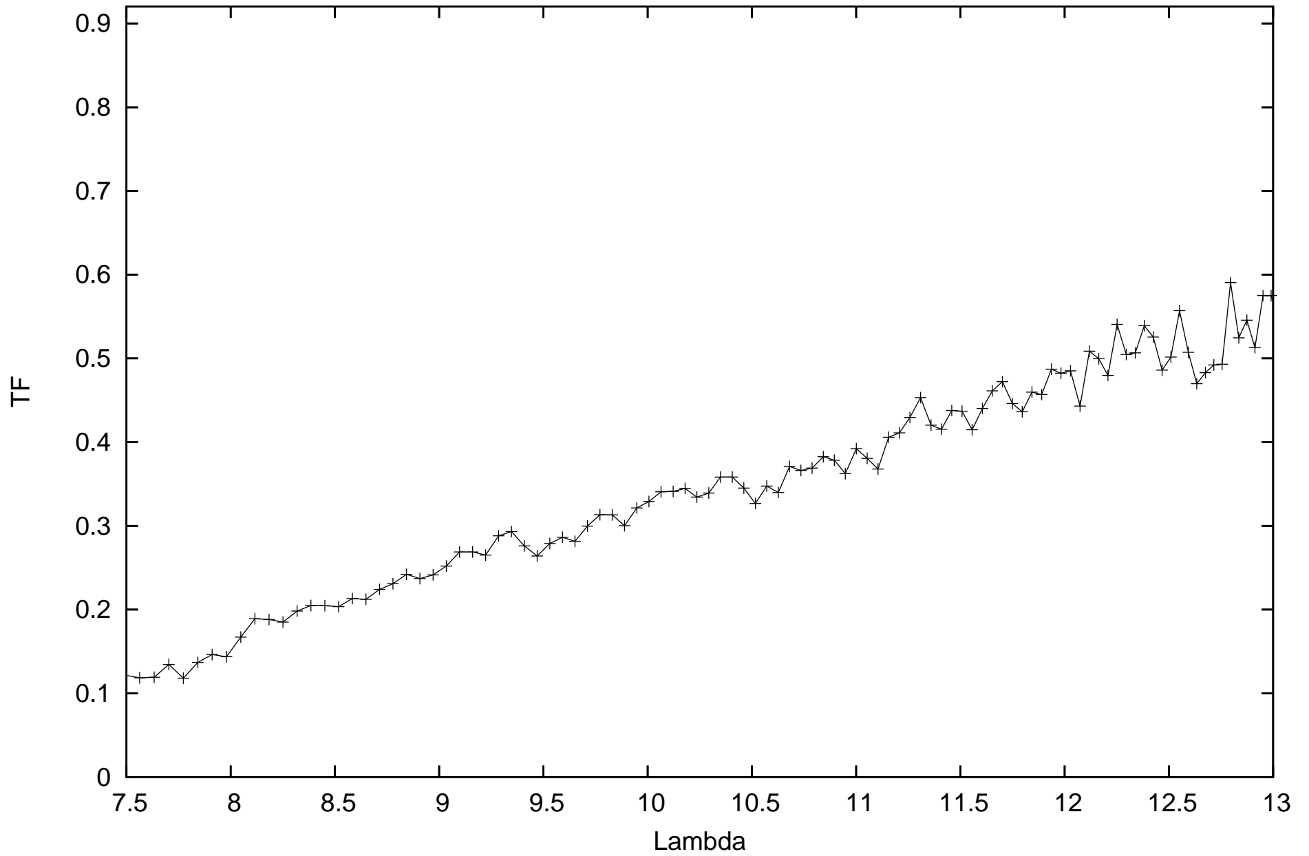
calHD167618_flux-1.82_diam11.66_r.MIDI.2013-09-16T00_21_16.112_H0D0
