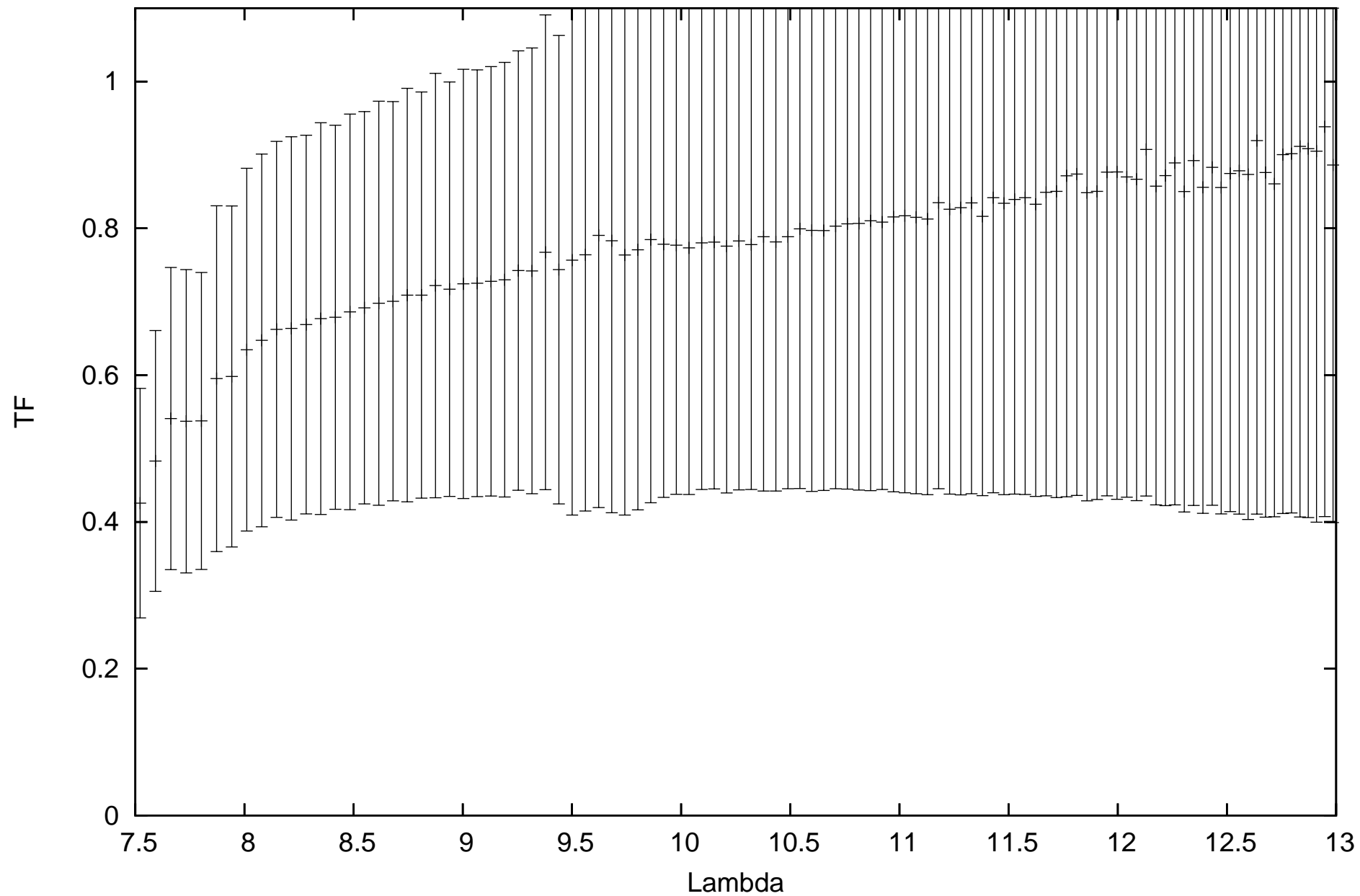
calHIP110997_flux1.58908_diam2.11_r.MIDI.2013-08-18T08_43_55.000_U3U4
