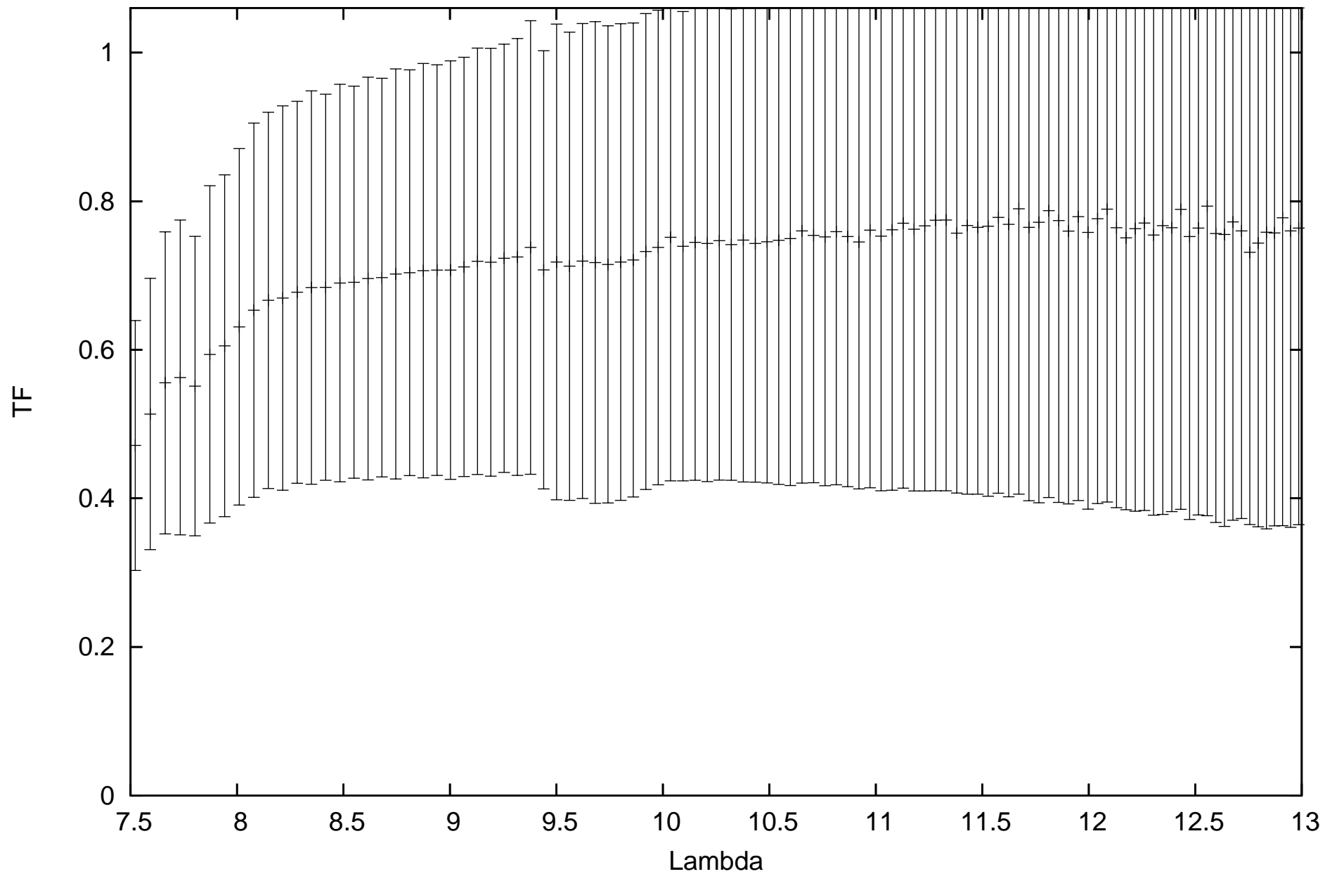
calHIP110997_flux1.58908_diam2.11_r.MIDI.2013-08-18T05_49_04.000_U3U4
