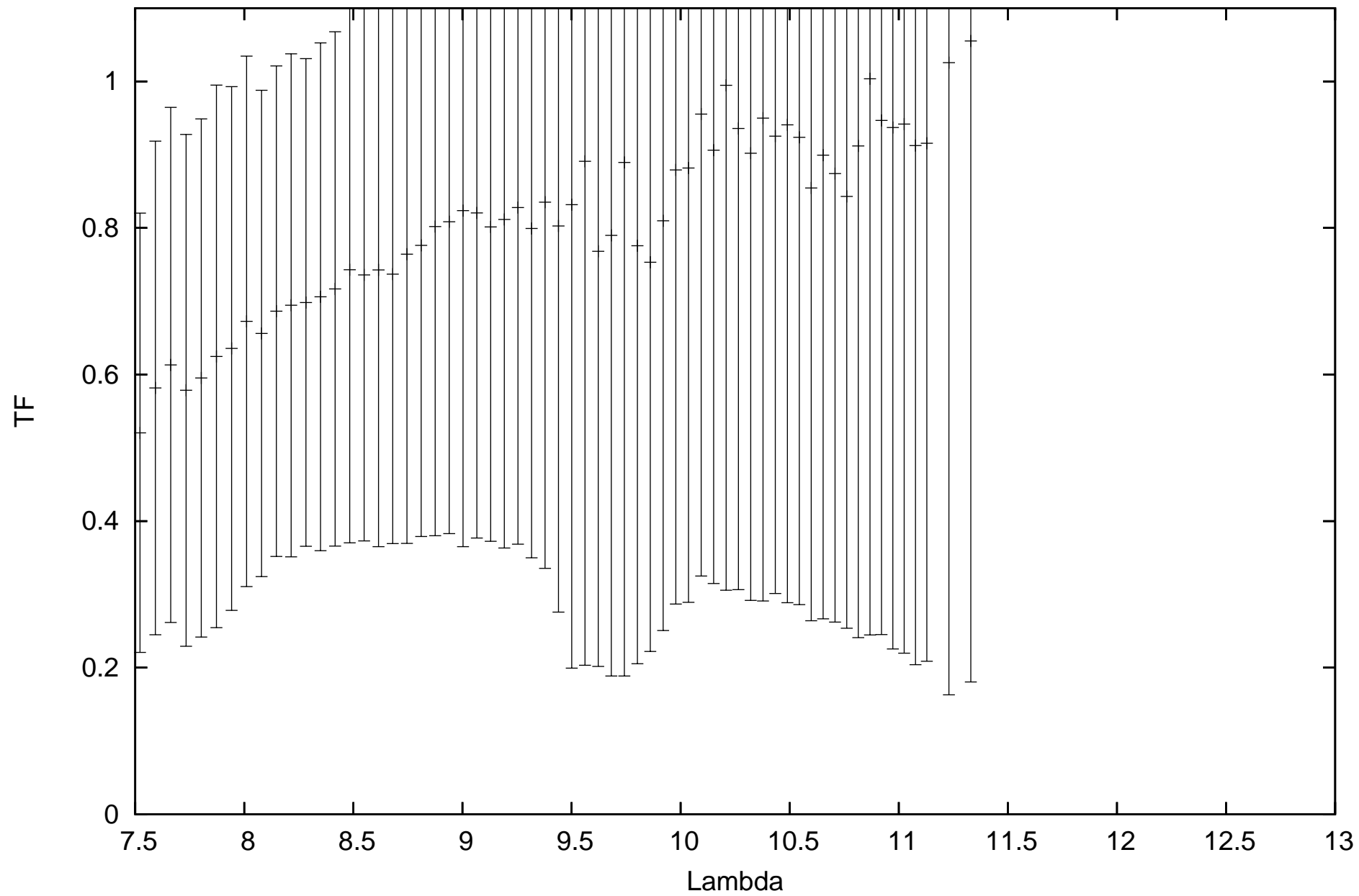
calHIP90496_flux0.238088_diam3.99_r.MIDI.2013-08-12T03_45_25.000_D0B2
