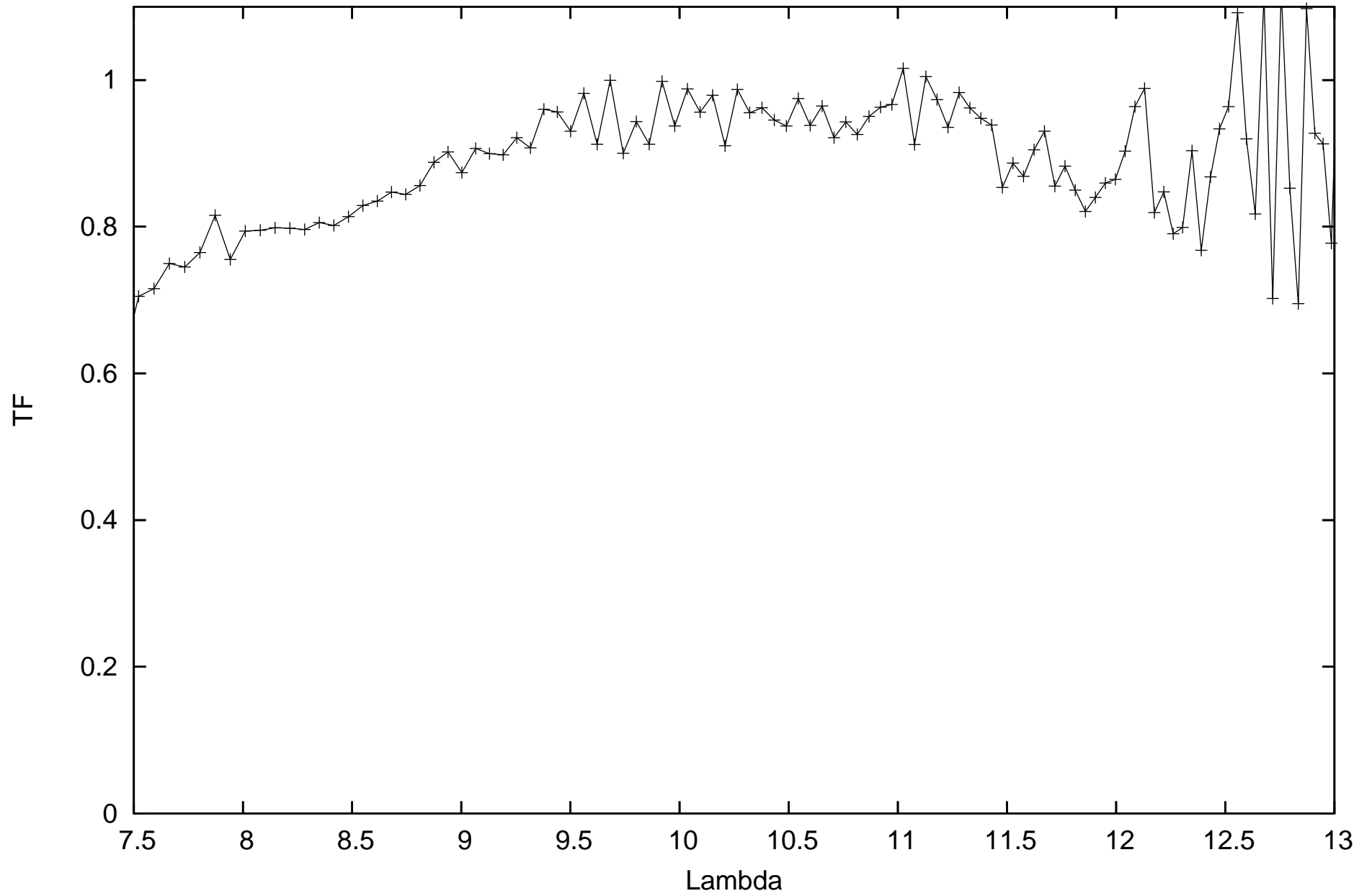
calHIP114724_flux0.200468_diam6.310939_r.MIDI.2013-08-12T09_10_38.000_C1B2
