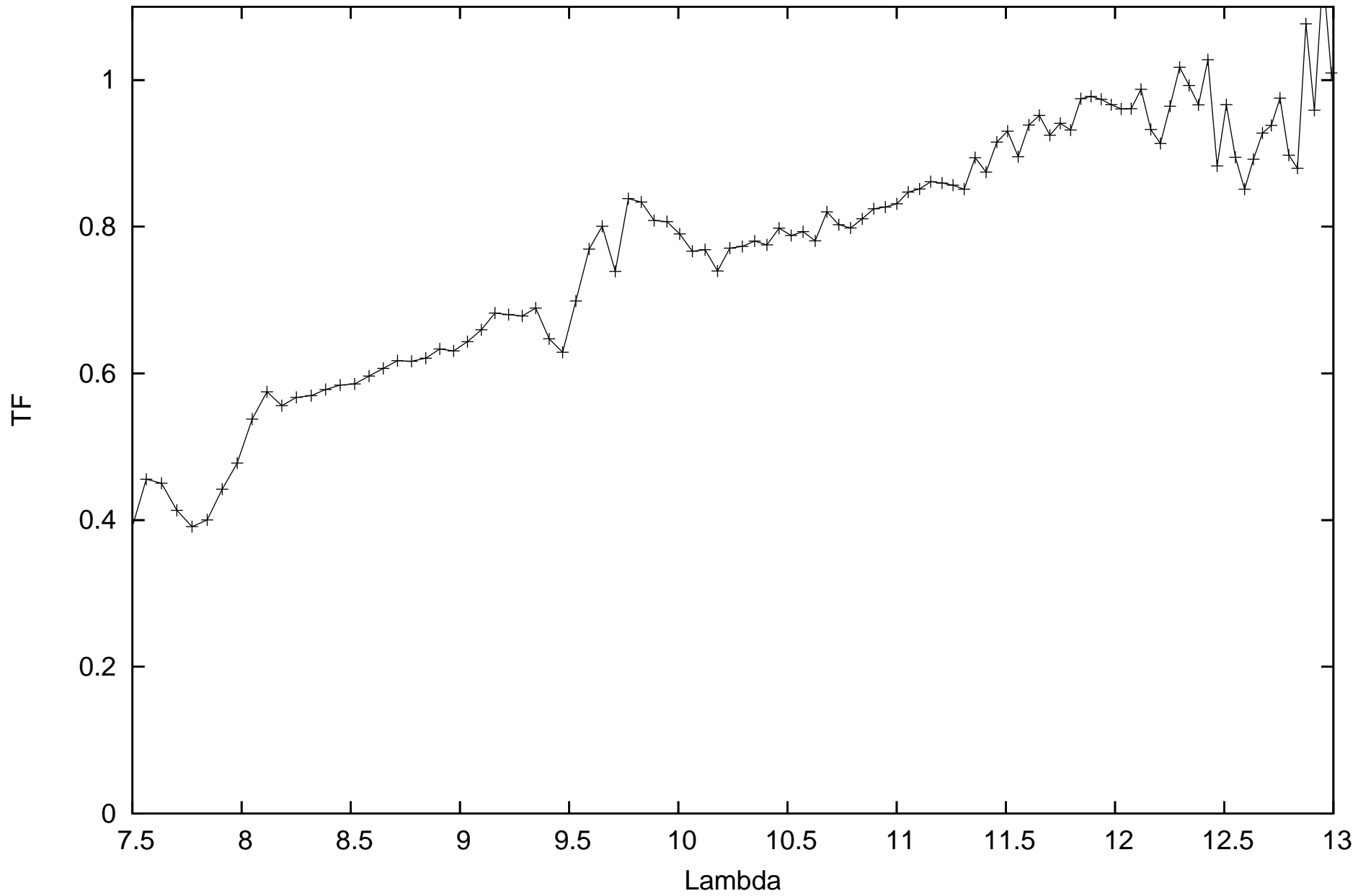
calHD167618_flux-1.82_diam11.66_r.MIDI.2013-08-06T07_04_20.113_D0B2
