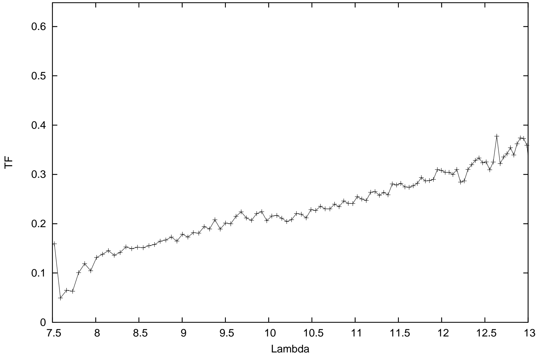
calHD167618_flux-1.82_diam11.66_r.MIDI.2013-07-30T07_31_17.000_D0B2
