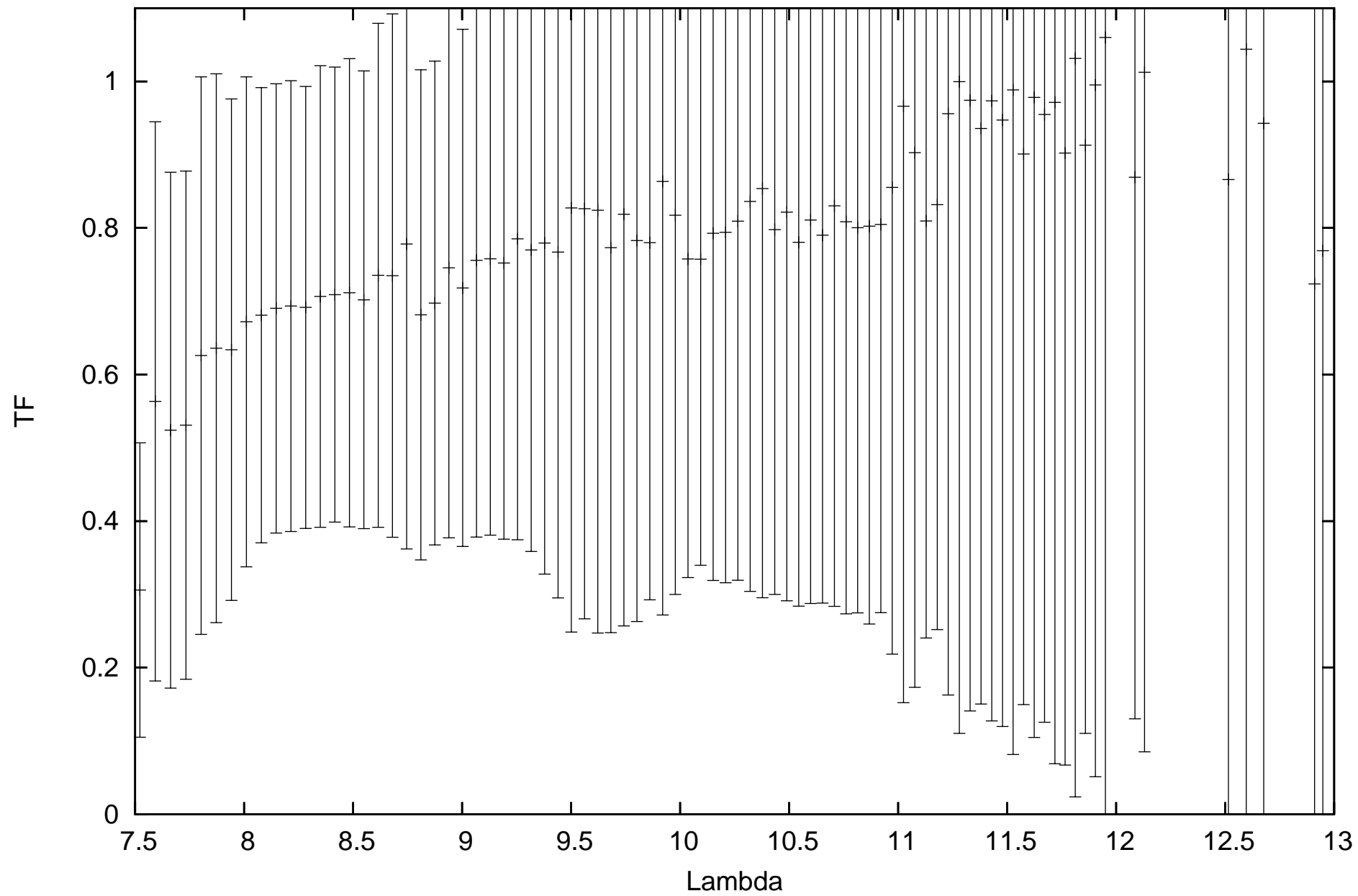
calHIP1170_flux-0.10766_diam5.17_r.MIDI.2013-07-29T08_52_46.000_G111
