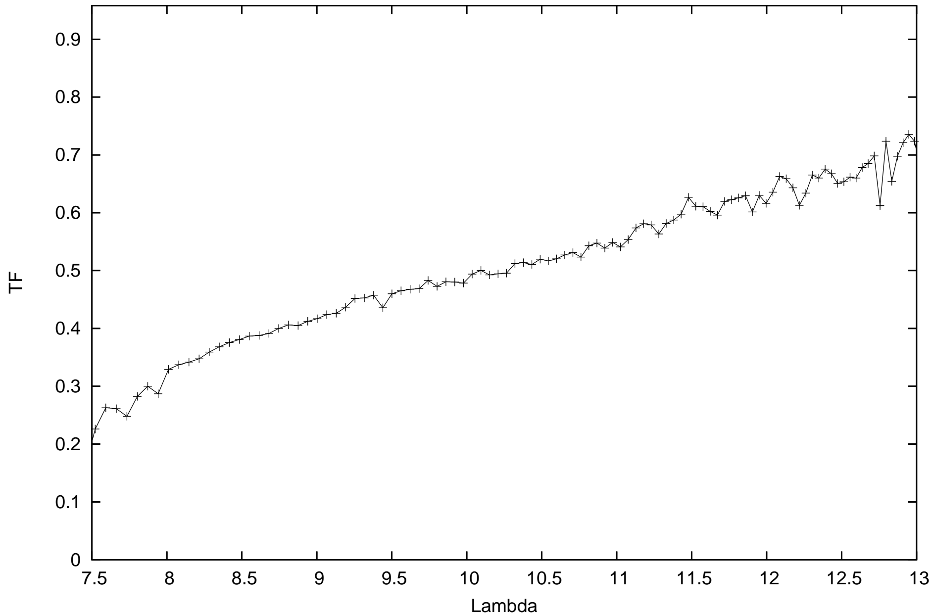
calHIP82273_flux-1.42243_diam8.91_r.MIDI.2013-07-28T03_07_47.000_G111
