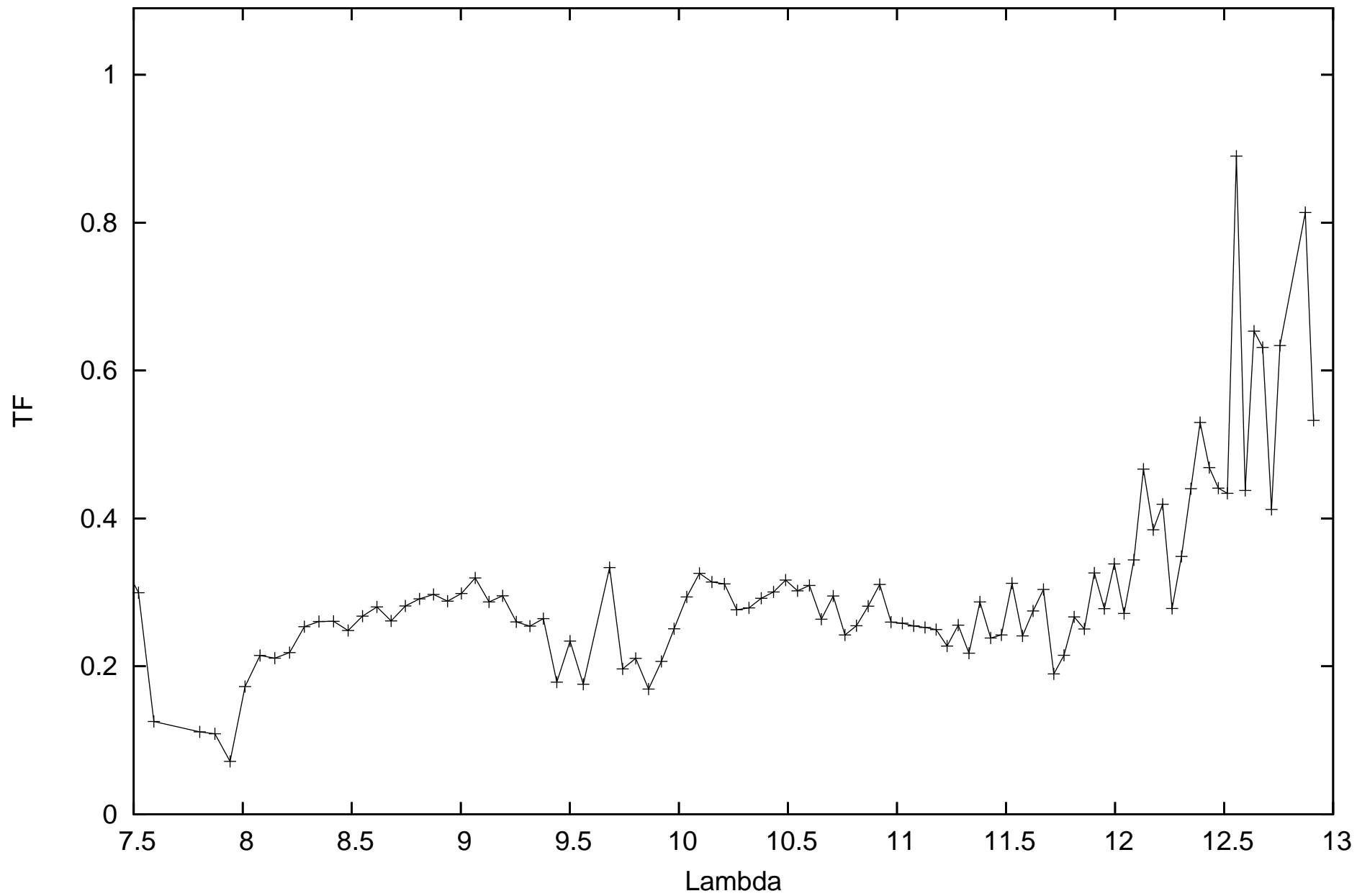
calHD125687_flux0.4_diam4.03_r.MIDI.2013-07-28T04_22_35.000_G111
