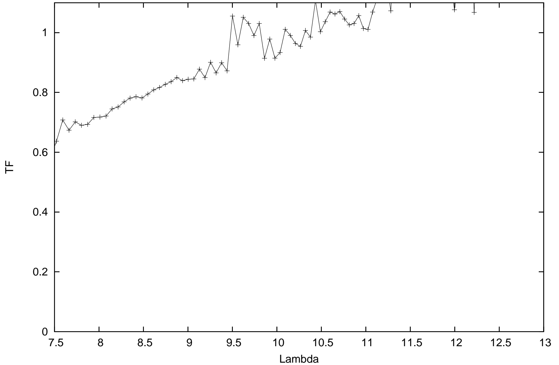
calHIP90496_flux0.238088_diam3.99_r.MIDI.2013-07-16T04_05_07.000_H011
