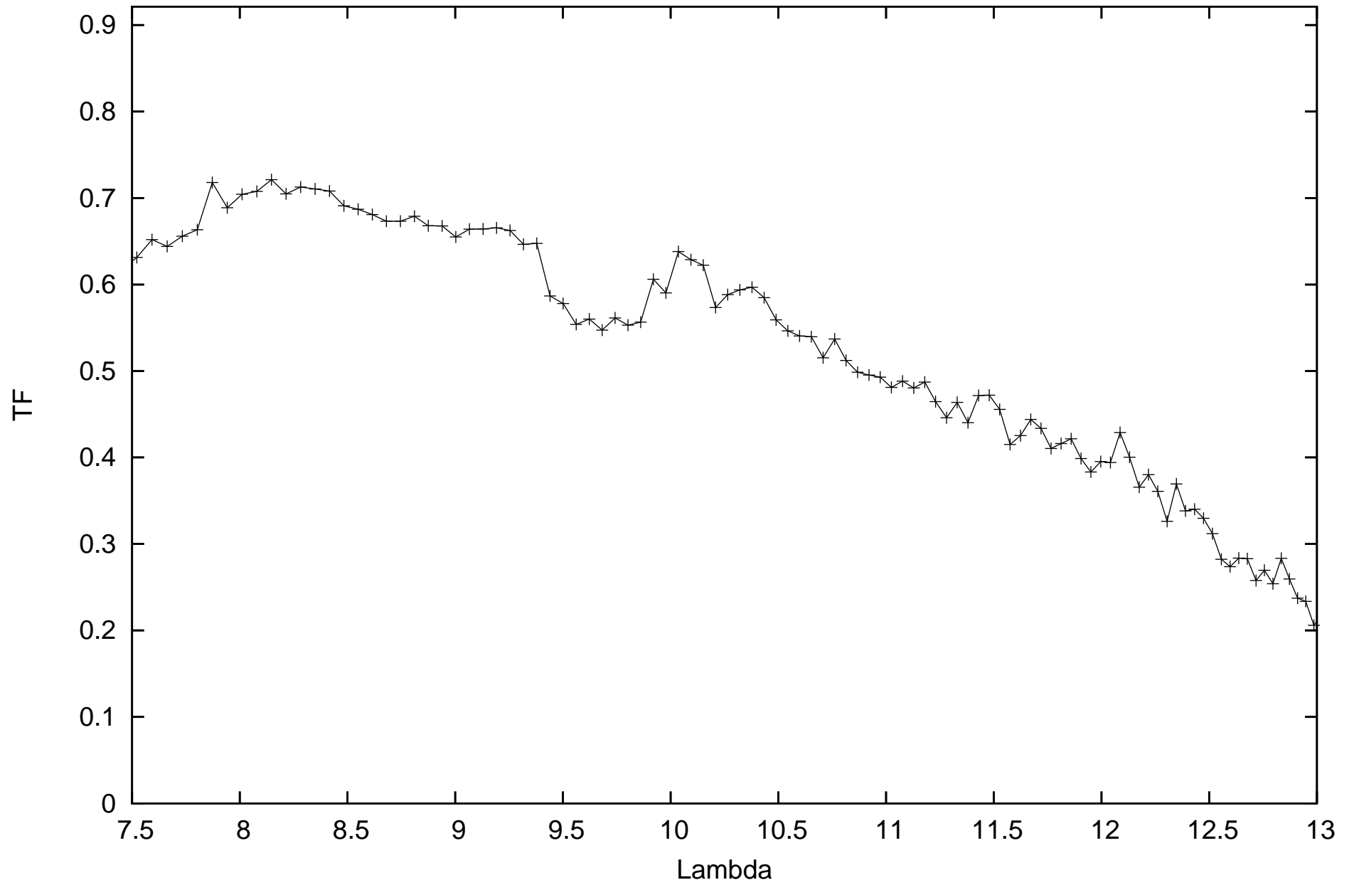
calHIP90496_flux0.238088_diam3.99_r.MIDI.2013-07-16T02_37_11.000_D0H0
