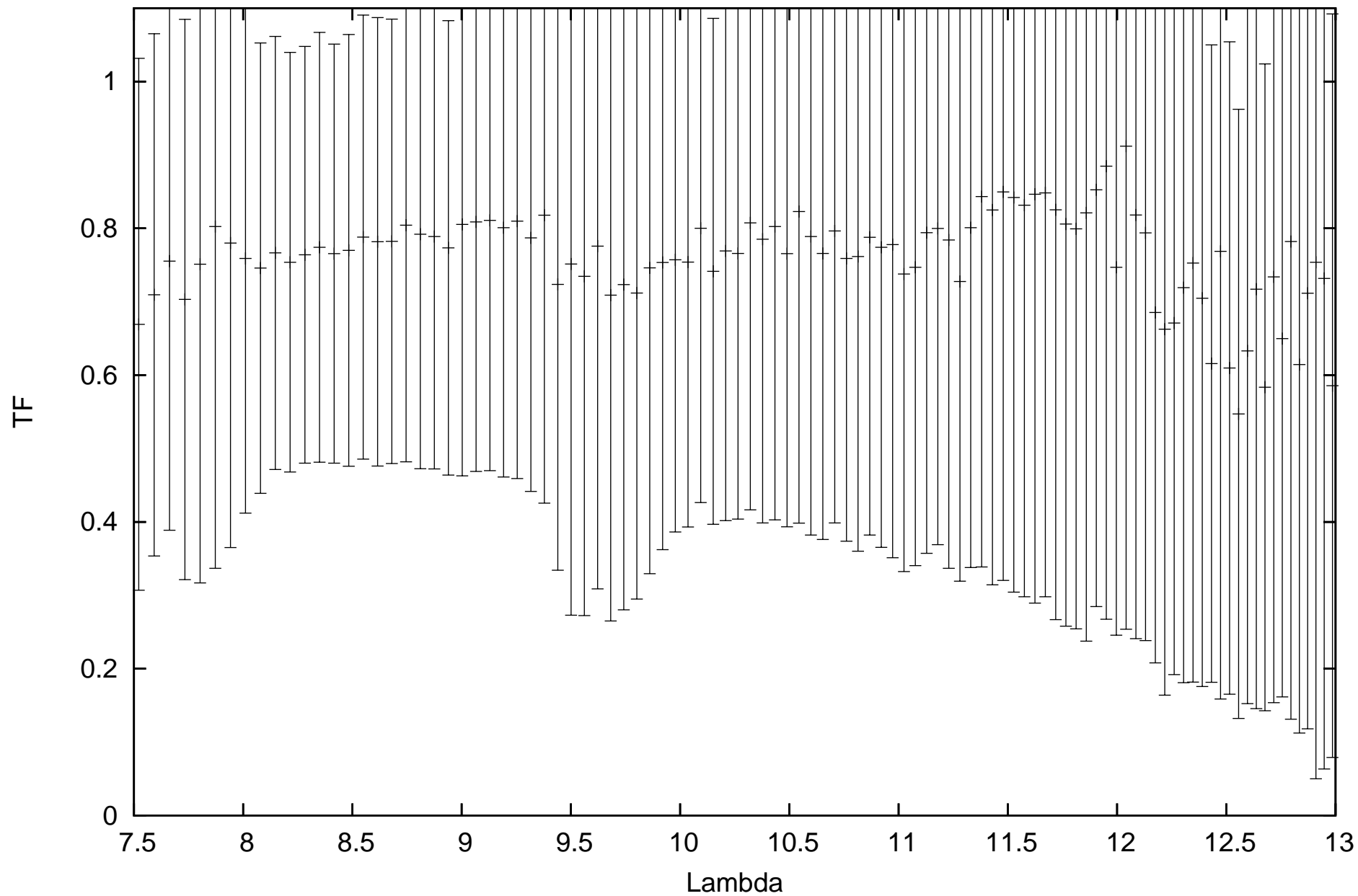
calHIP104234_flux0.336362_diam4.534747_r.MIDI.2013-07-16T09_45_48.000_H011
