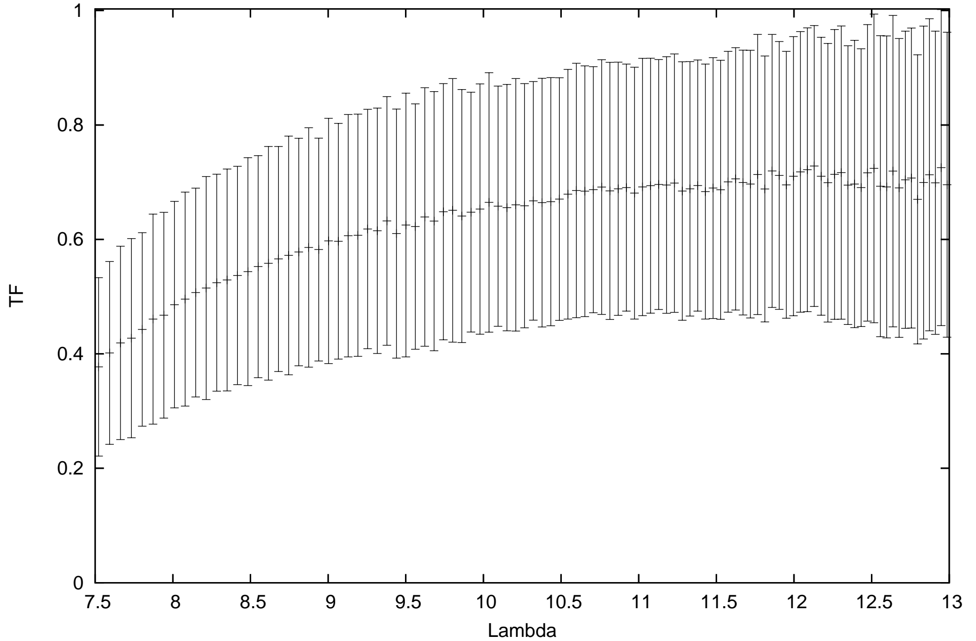
calHD167618_flux-1.82_diam11.66_r.MIDI.2013-07-13T01_35_19.000_D011
