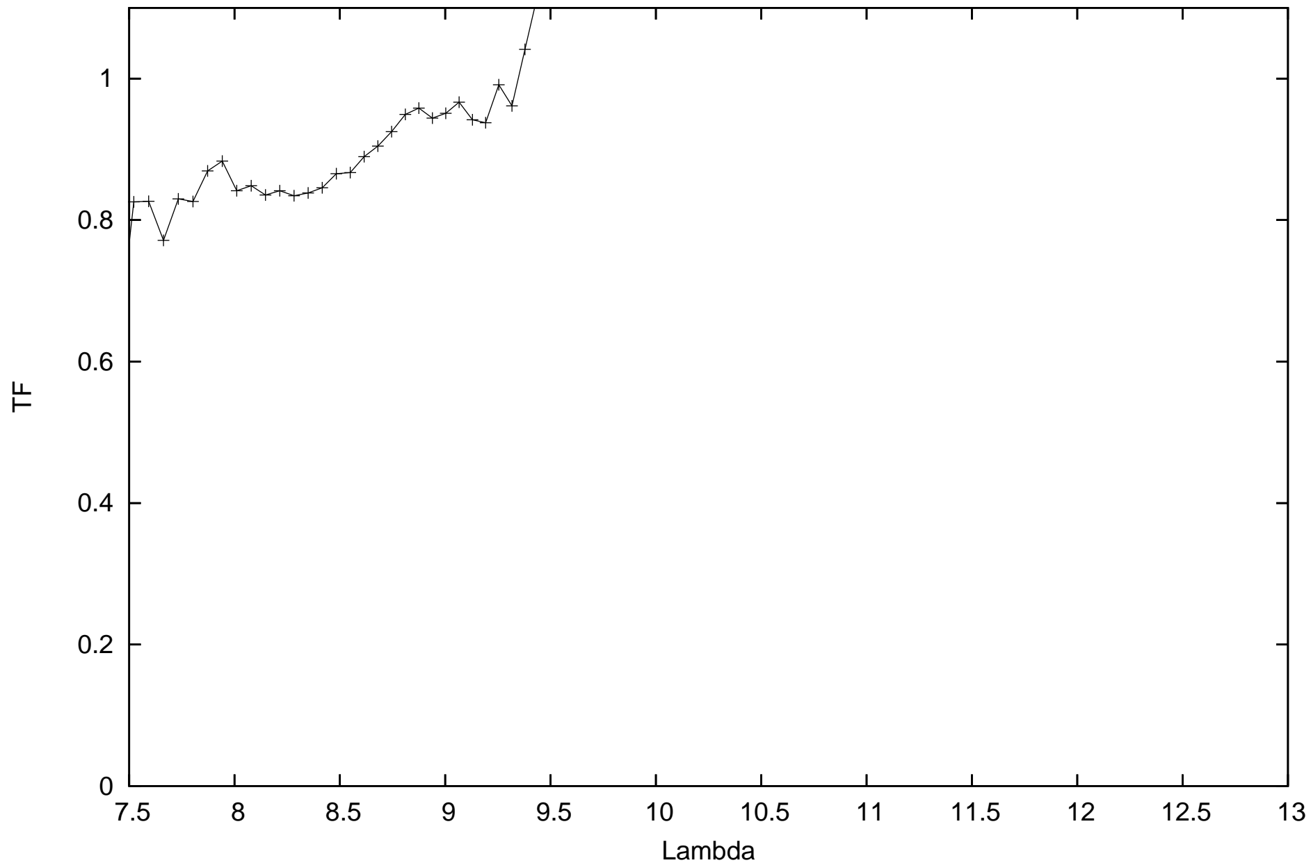
calHIP90496_flux0.238088_diam3.99_r.MIDI.2013-07-12T06_34_17.000_K0J3
