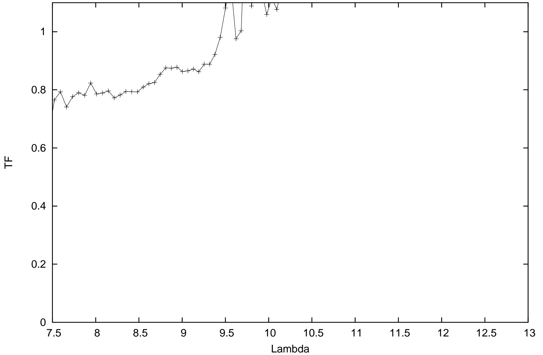
calHIP90496_flux0.238088_diam3.99_r.MIDI.2013-07-12T06_06_09.000_K0J3
