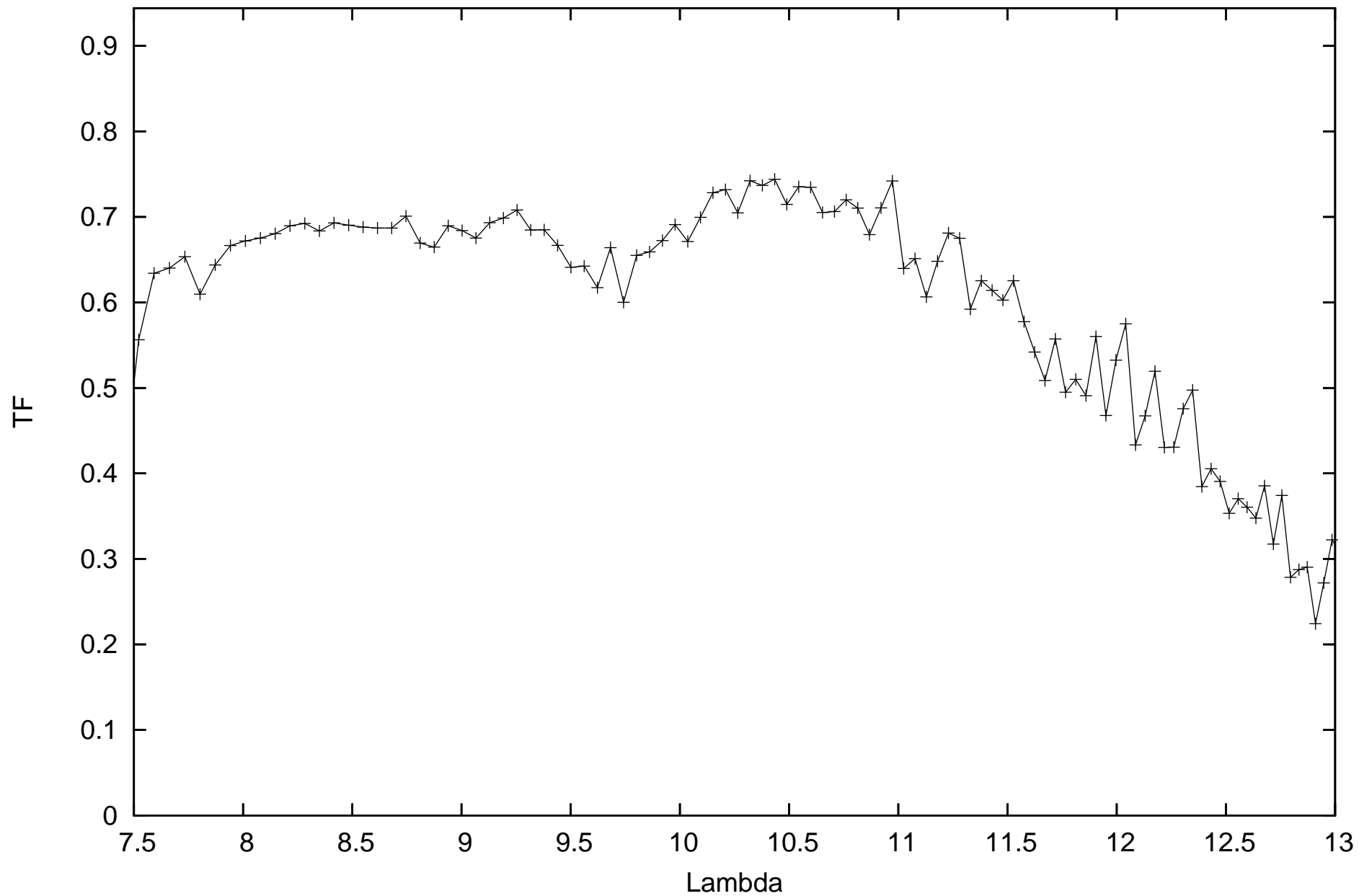
calHIP90496_flux0.238088_diam3.99_r.MIDI.2013-07-12T02_44_22.000_G1A1
