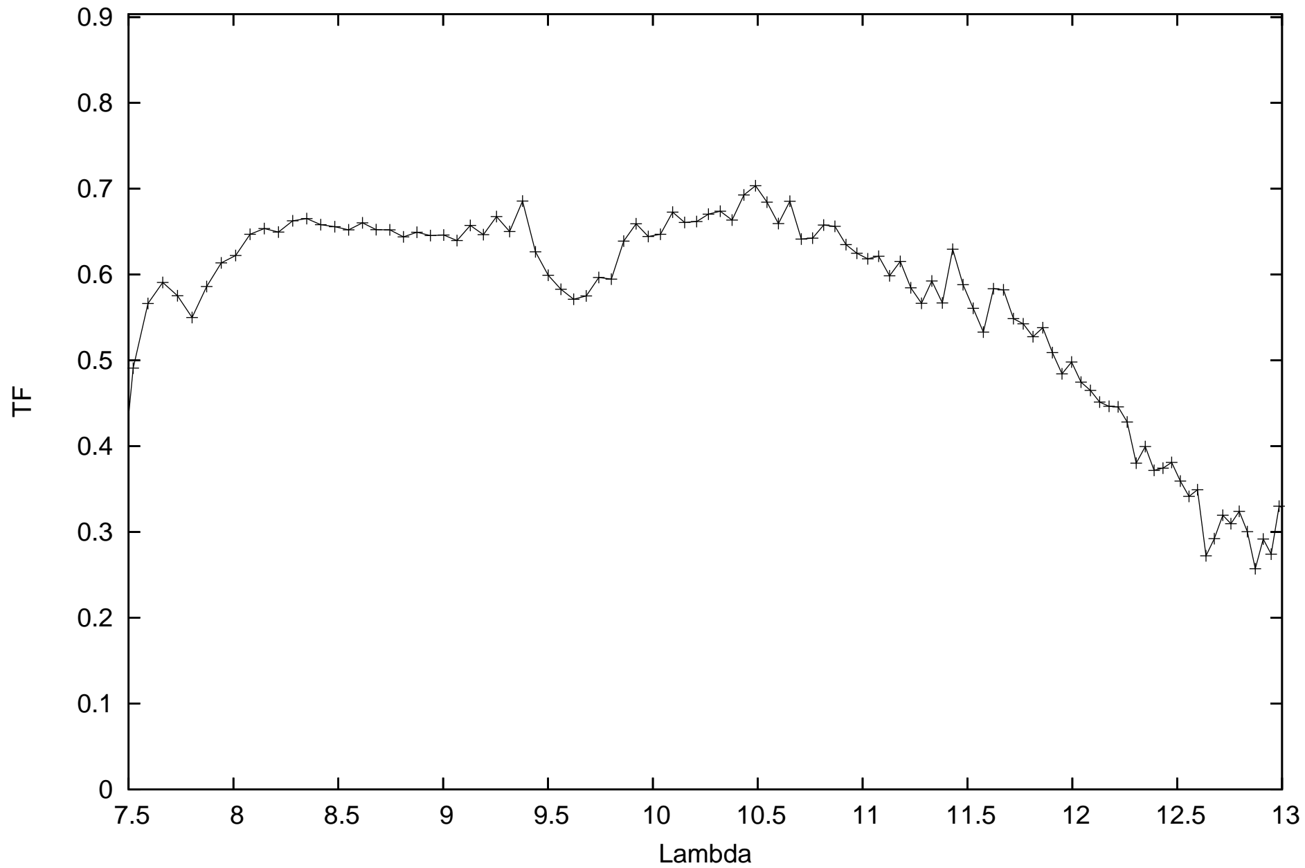
calHIP90496_flux0.238088_diam3.99_r.MIDI.2013-07-12T01_52_49.000_K0G1
