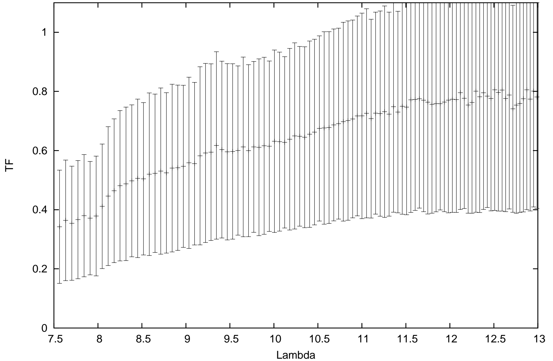
calHIP73714_flux-1.78451_diam11.15_r.MIDI.2013-06-19T01_13_58.947_U2U3
