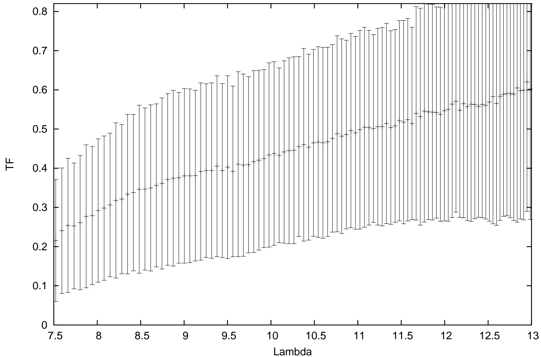
calHD167618_flux-1.82_diam11.66_r.MIDI.2013-06-12T04_43_27.000_H0G1
