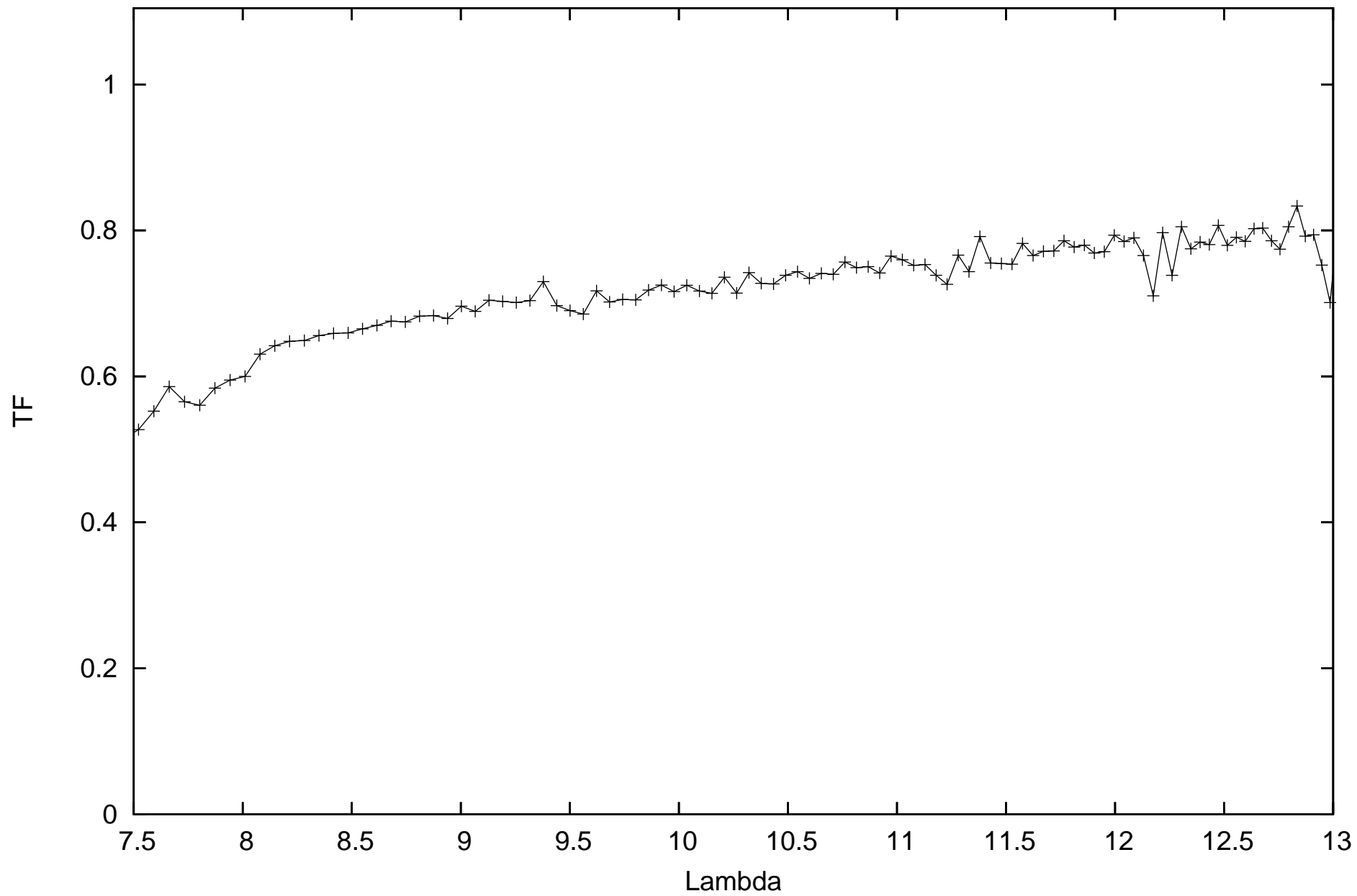
calHD173074_flux1.59_diam2.5_r.MIDI.2013-05-03T09_11_26.000_U1U2
