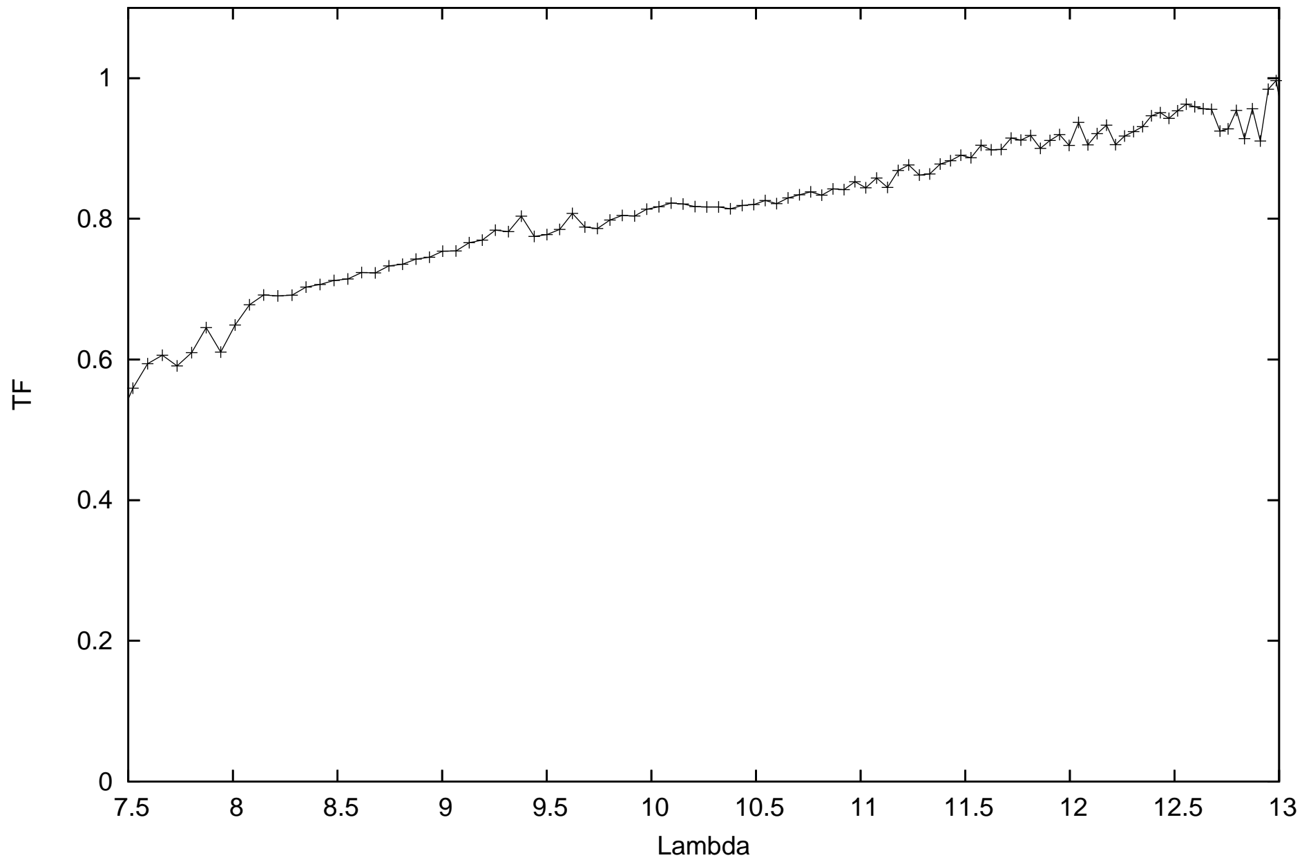
calHD168723_flux0.9_diam2.91_r.MIDI.2013-04-30T07_49_46.000_U1U4
