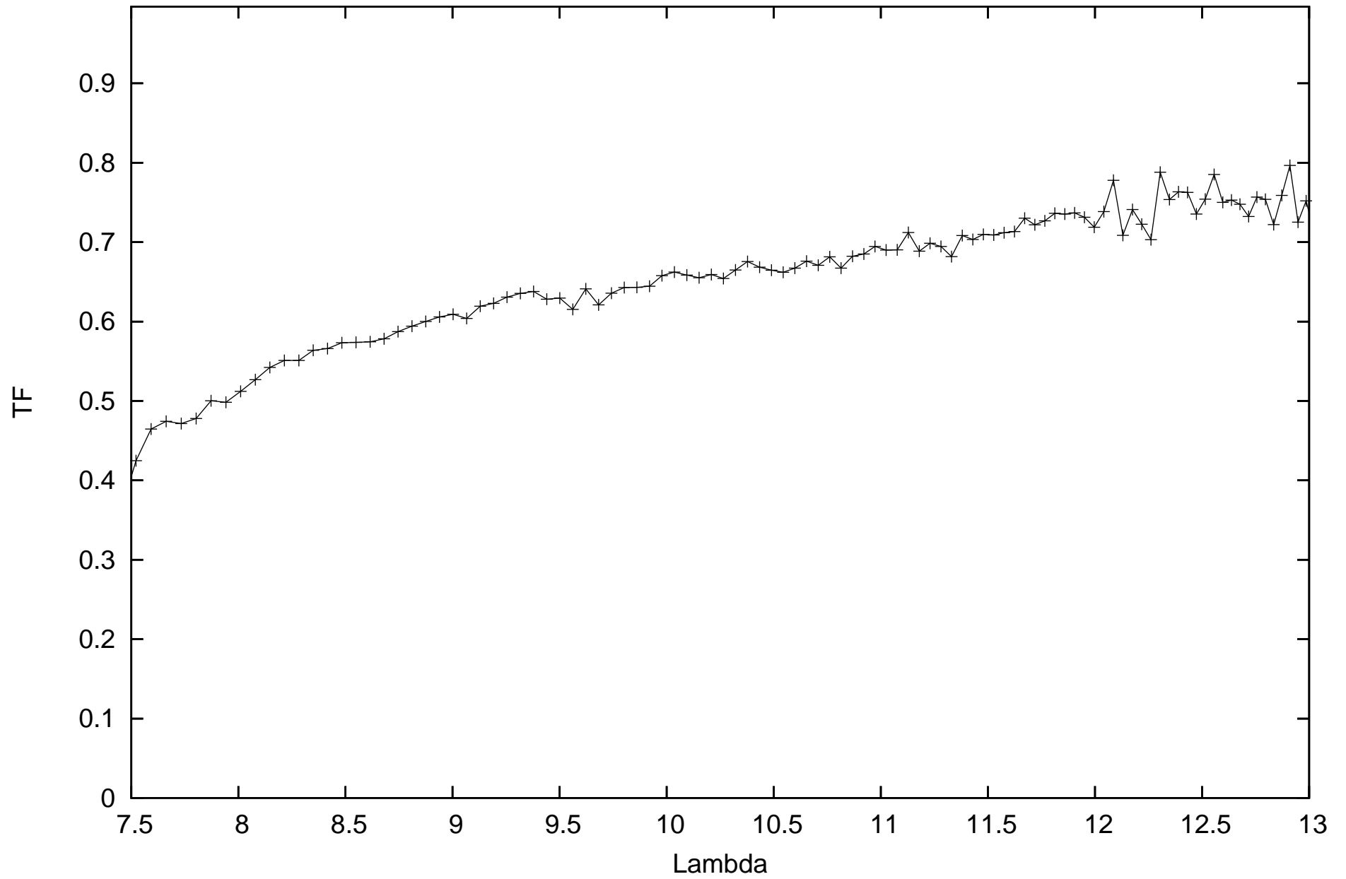
calHIP79593_flux-1.46675_diam10.14017_r.MIDI.2013-04-26T07_03_20.000_H0G1
